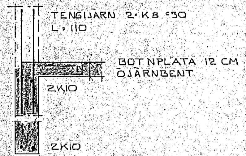
SNID I UNDIRST.VEGG M 1:20
