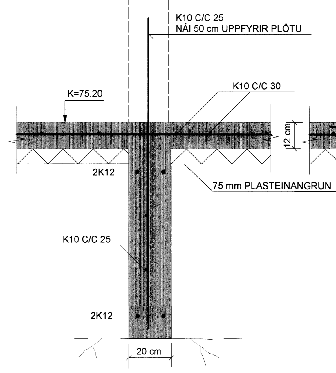
SNID F-F MKV. 1:10
