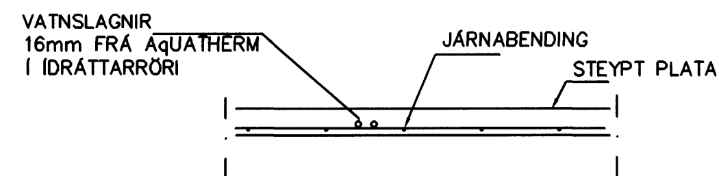
LAGNIR, SNID, 1:20
