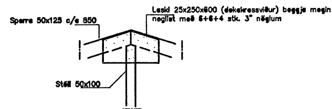
SNID 6-6 1:20
