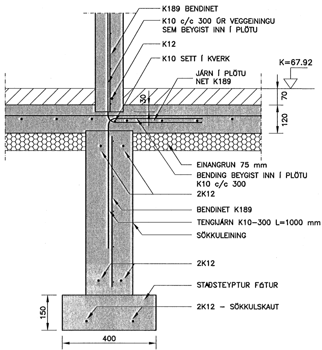
SNID 2-2 1:10
