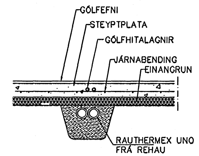
LAGNIR, SNID, 1:20
