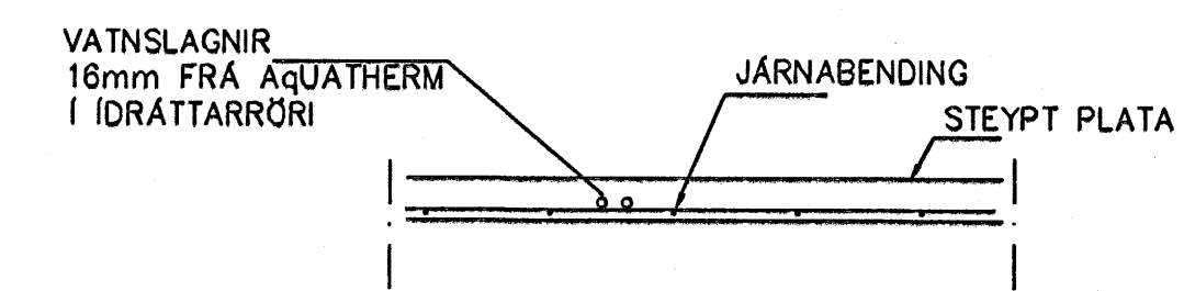
LAGNIR, SNID, 1:20
