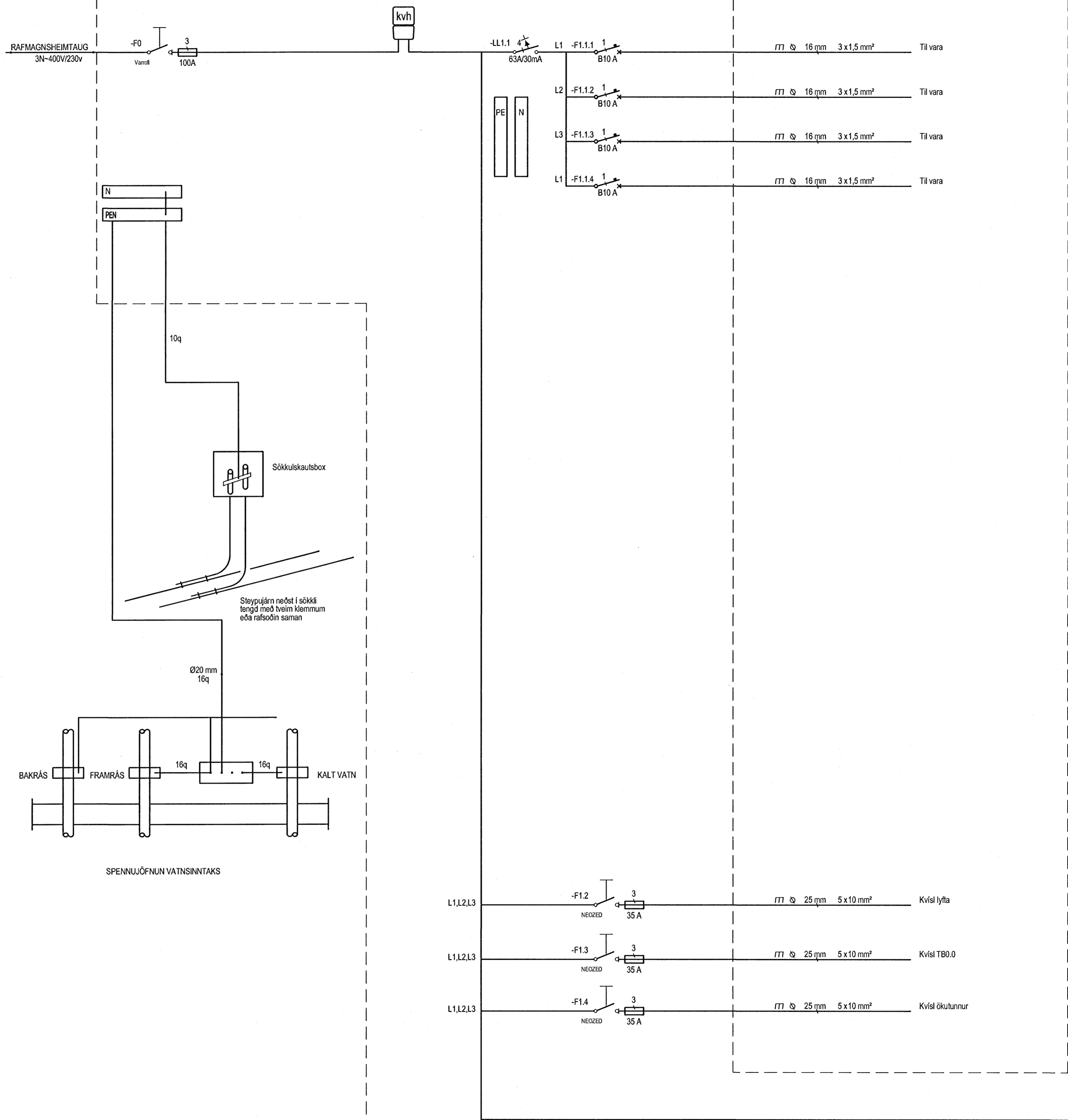
Aðaltafla T0.0 TN-C-S 400/230 Vac
