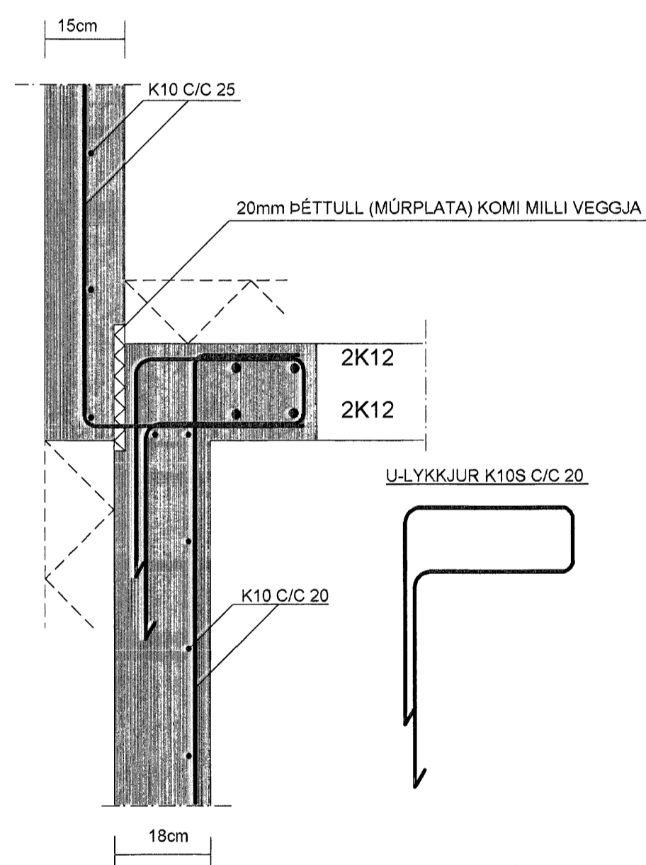
SNID 10-10 MKV. 1:10
