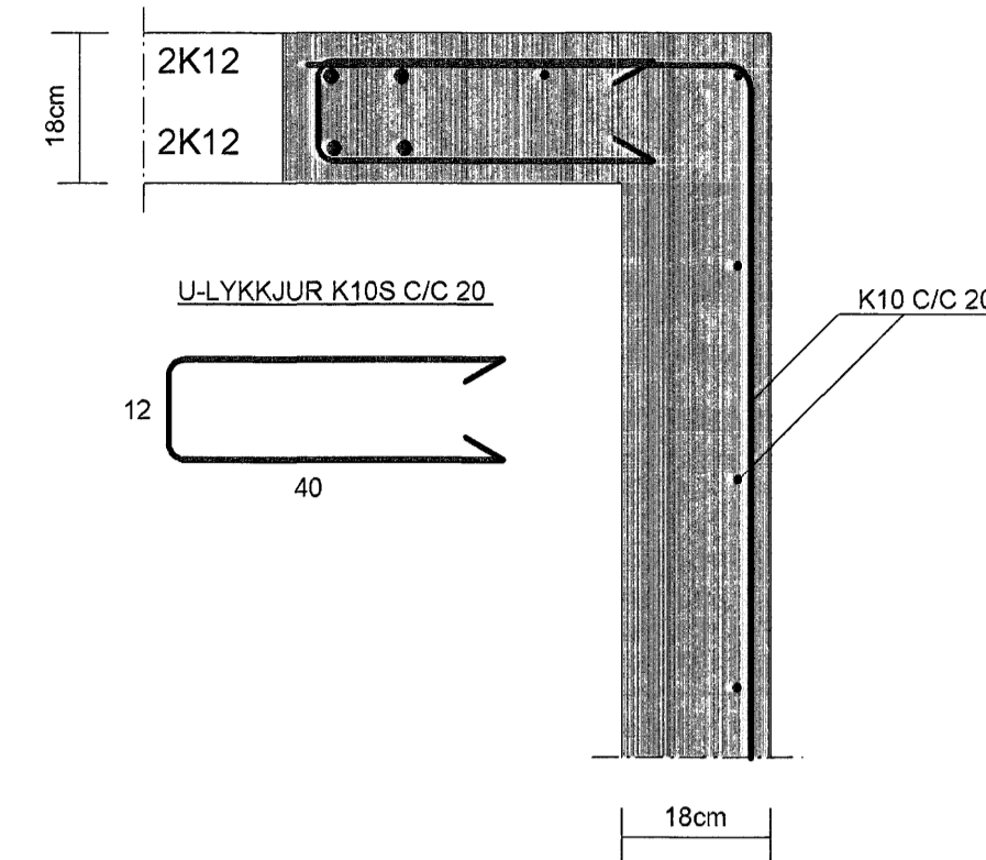
SNID 8-8 MKV. 1:10
