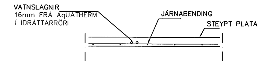
LAGNIR, SNID, 1:20
