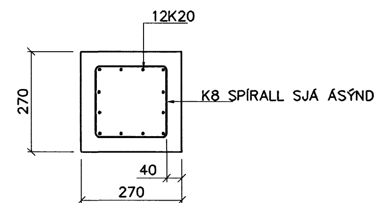
SNID B 1:10
