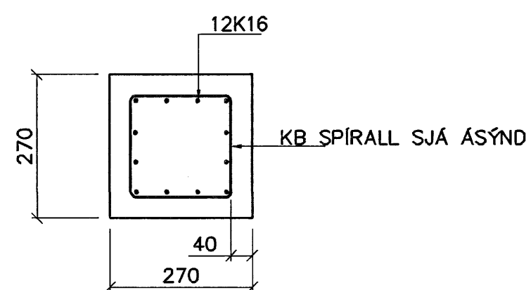
SNID A 1:10
