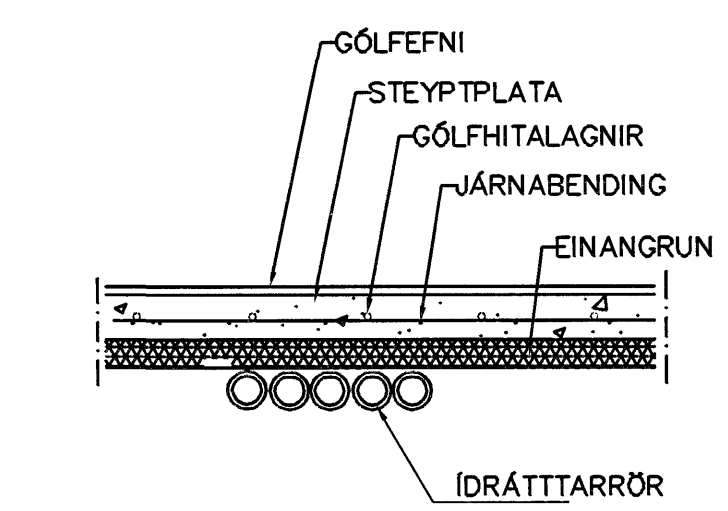
LAGNIR, SNIB, 1:20
