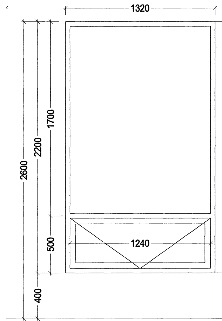
G9 1.stk Hornluggi
