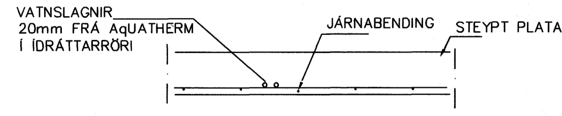
LAGNIR, SNID, 1:20
