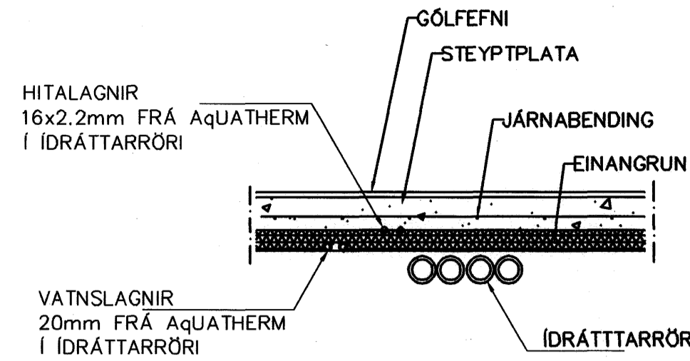
LAGNIR, SNID, 1:20
