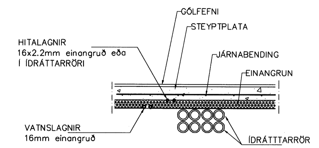
LAGNIR, SNID, 1:20
