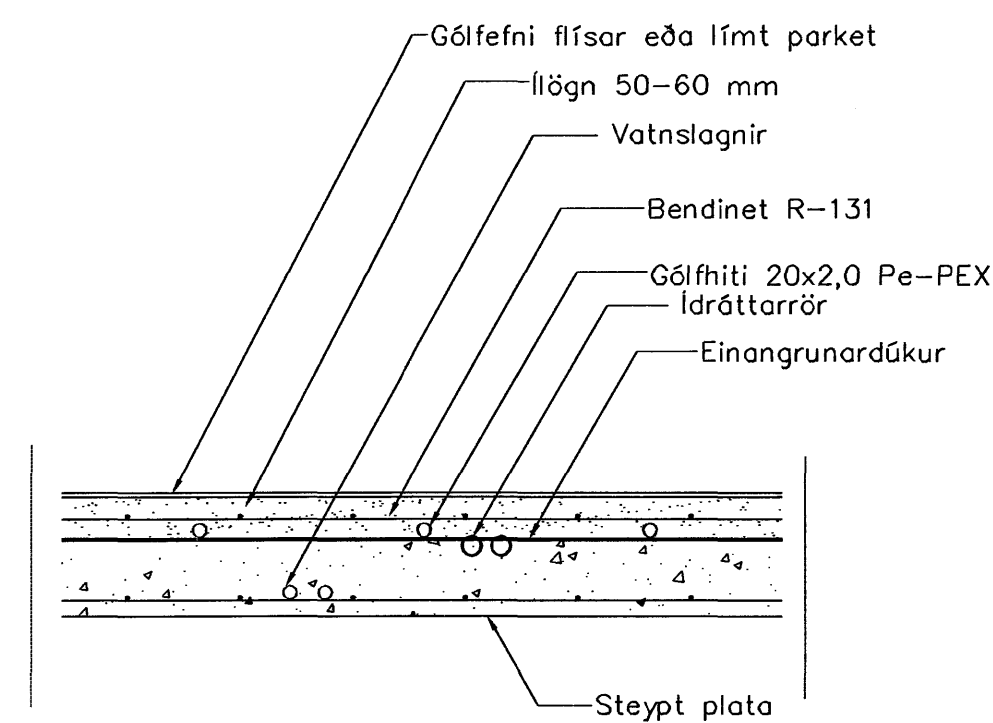
LAGNIR, SNID, 1:20
