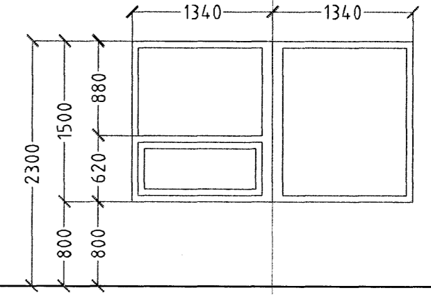
1 STK. Hjón Björgunarop Horngluggi
