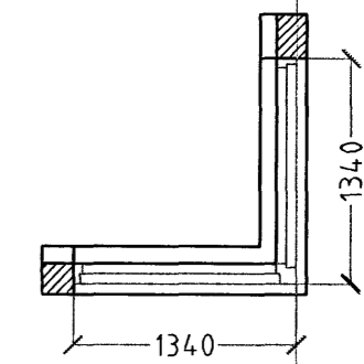
1 STK. Hjón Björgunarop Horngluggi
