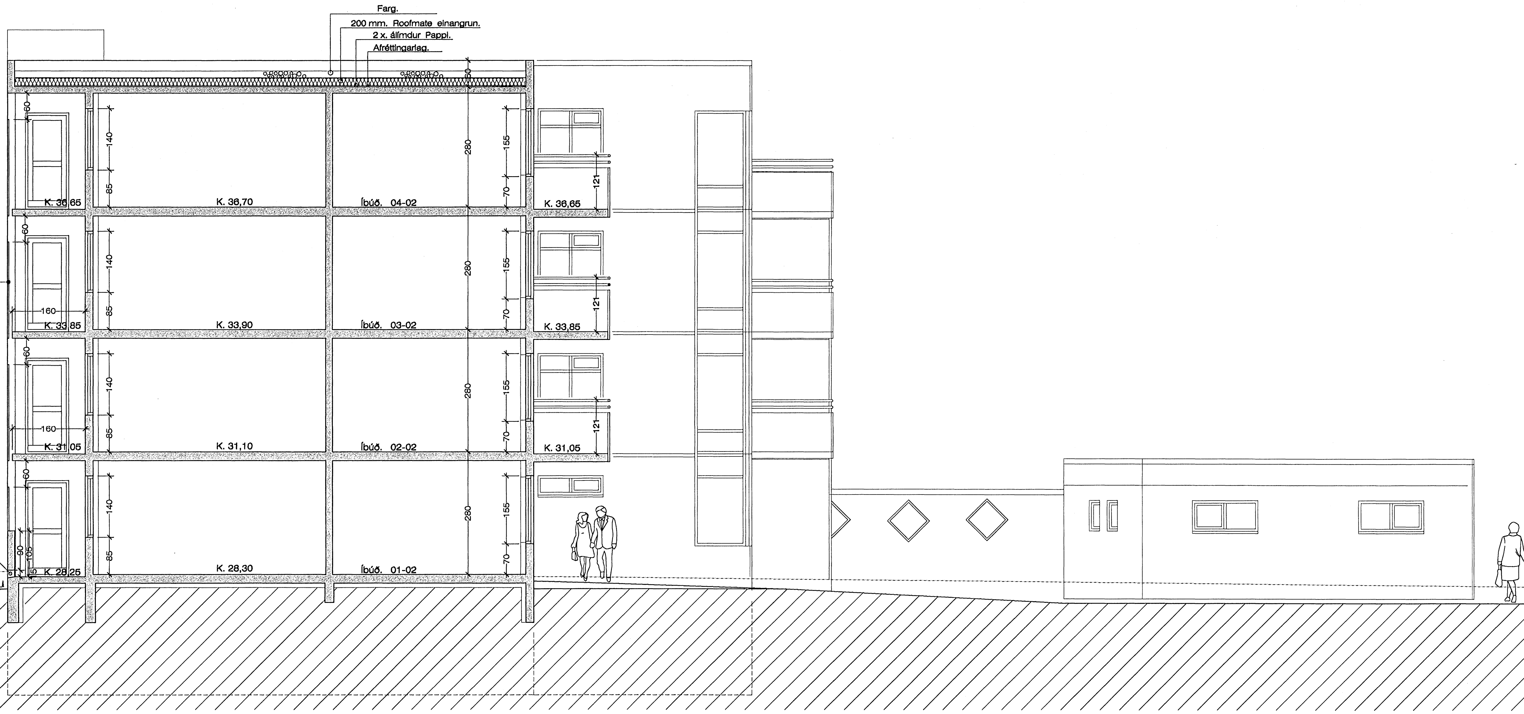
Sneiðing. C - C 1 : 50
