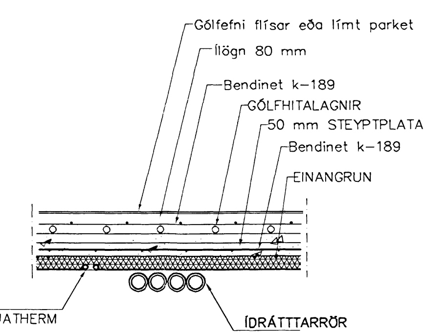
LAGNIR, SNID, 1:20
