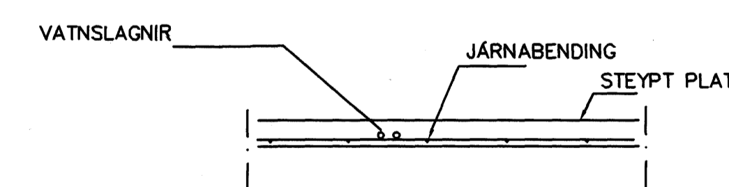
LAGNIR, SNID, 1:20
