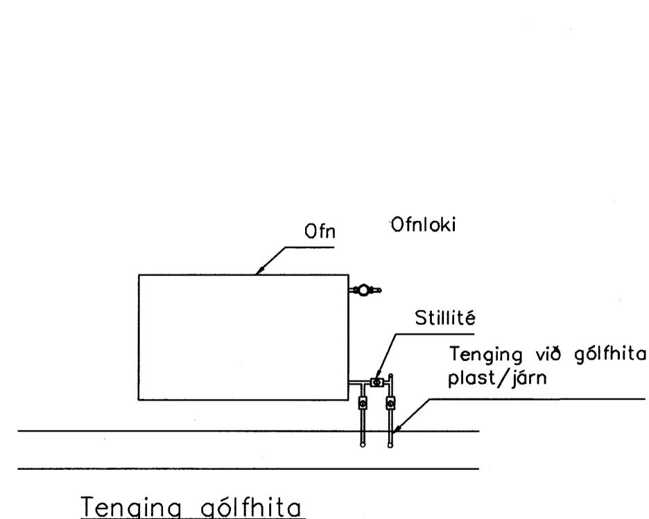
Tenging gölfhita
