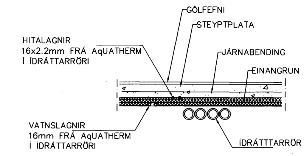
LAGNIR, SNID, 1:20
