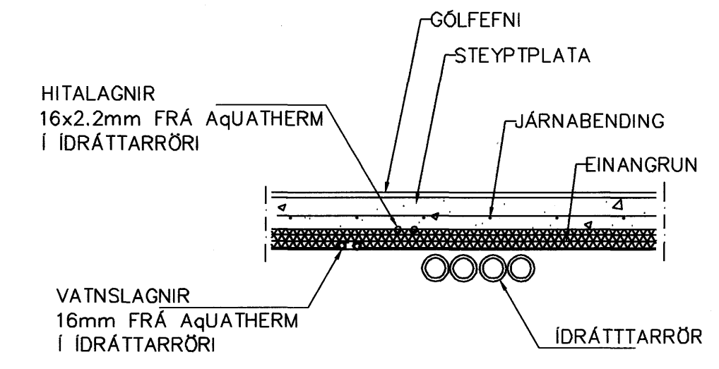
LAGNIR, SNID, 1:20
