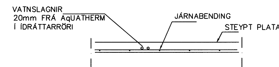
LAGNIR, SNID, 1:20
