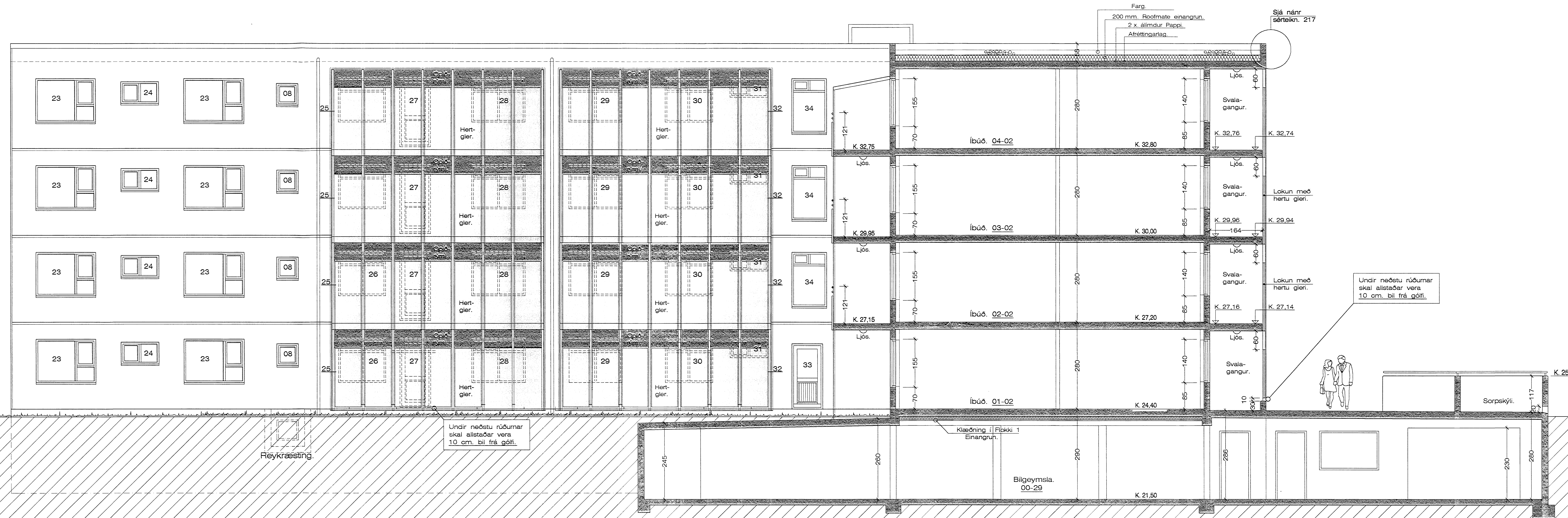
Sneiðing. B - B 1 : 50
