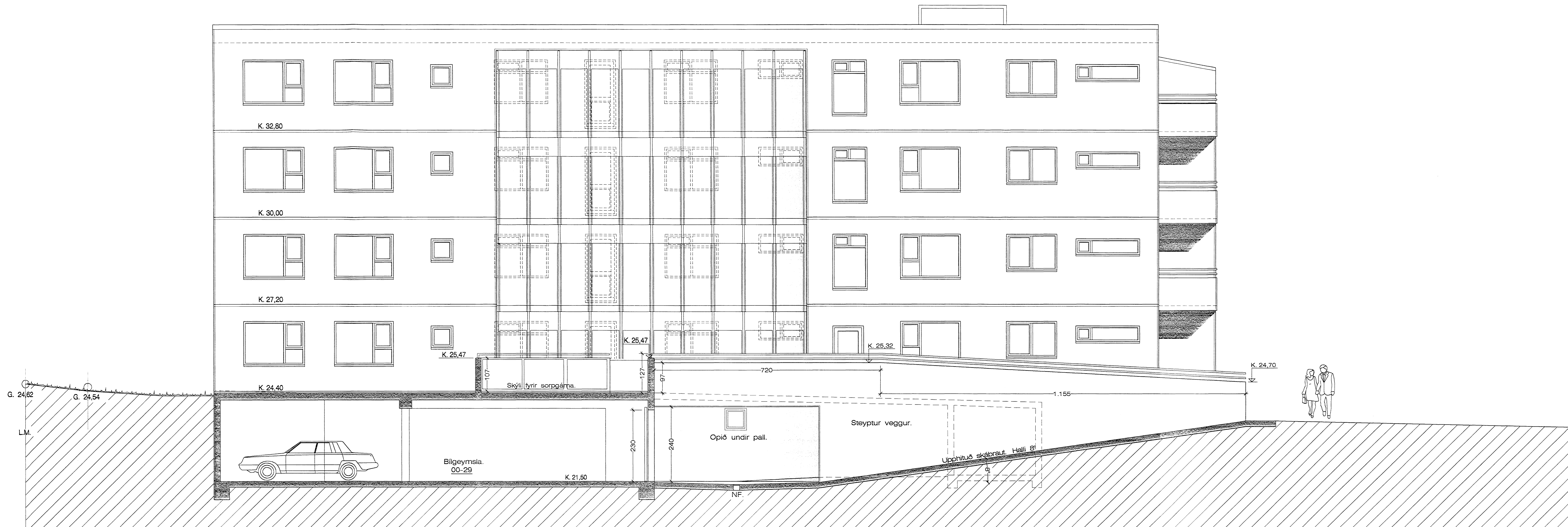
Sneiðing. D - D 1 : 50
