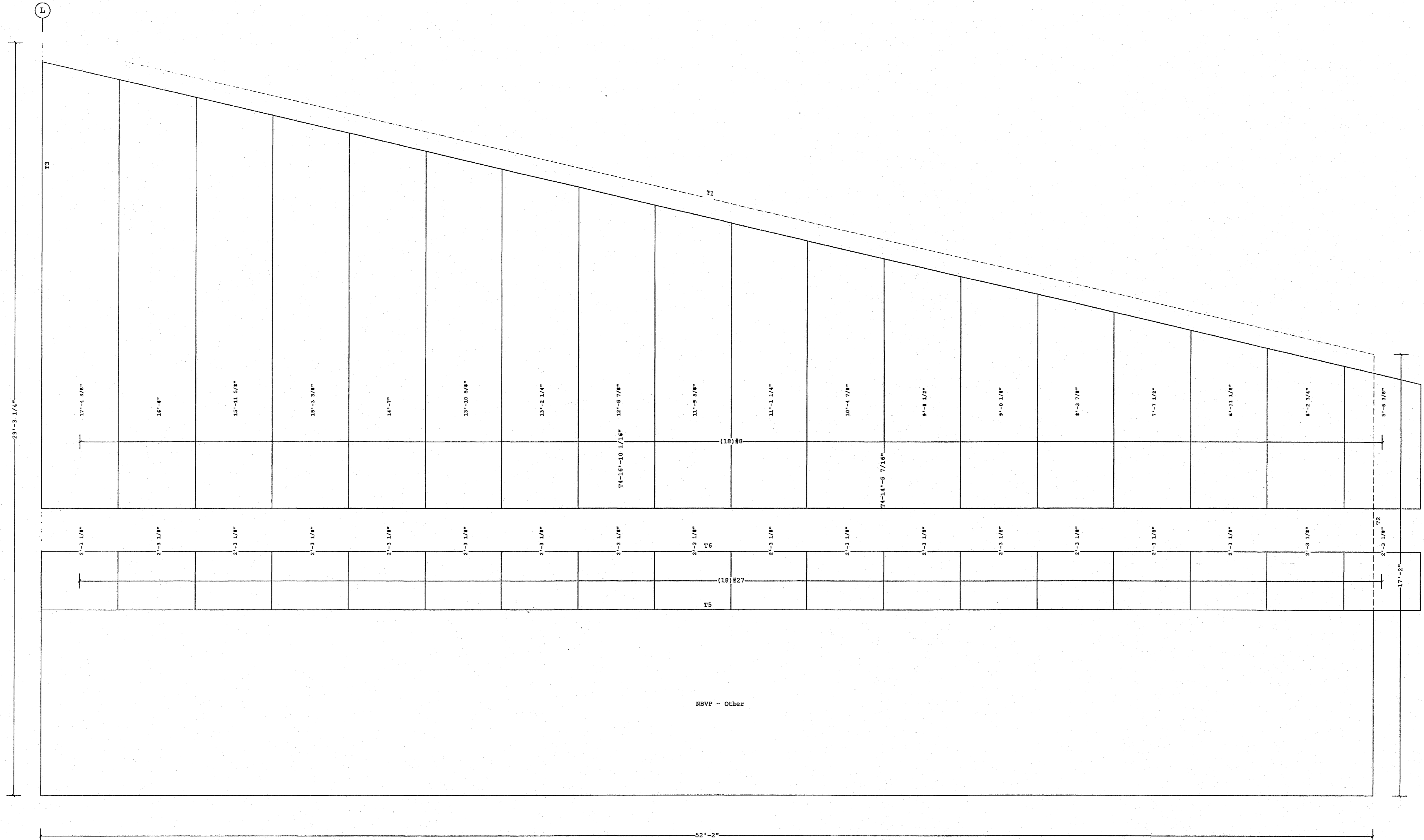
WALL LINER ELEVATION PARTITION OR MISC. 3 (View from inside Building)
