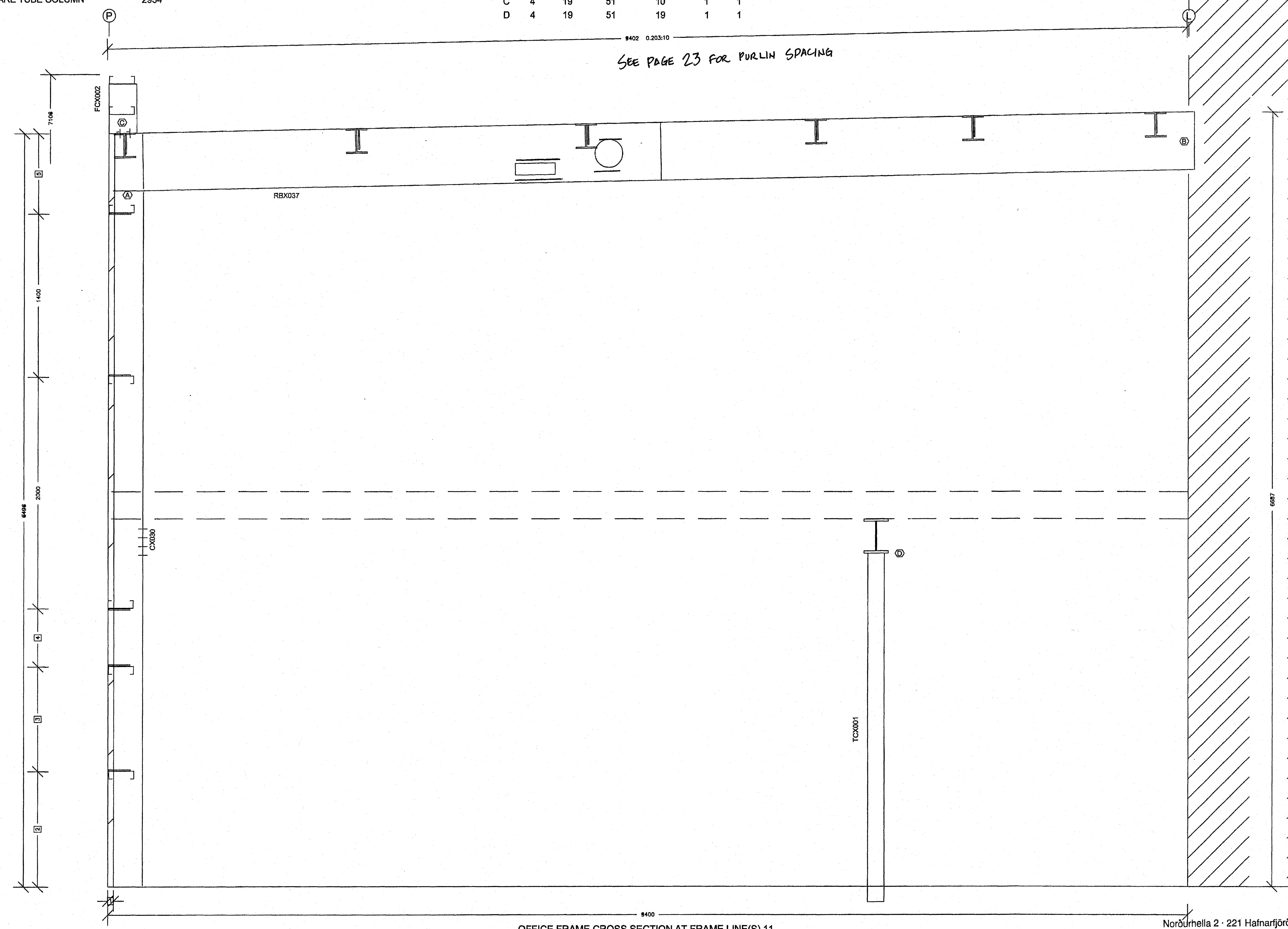
OFFICE FRAME CROSS SECTION AT FRAME LINE(S) 11 VP Ref: Shape Name = Office area Wall 6, Frame 10
