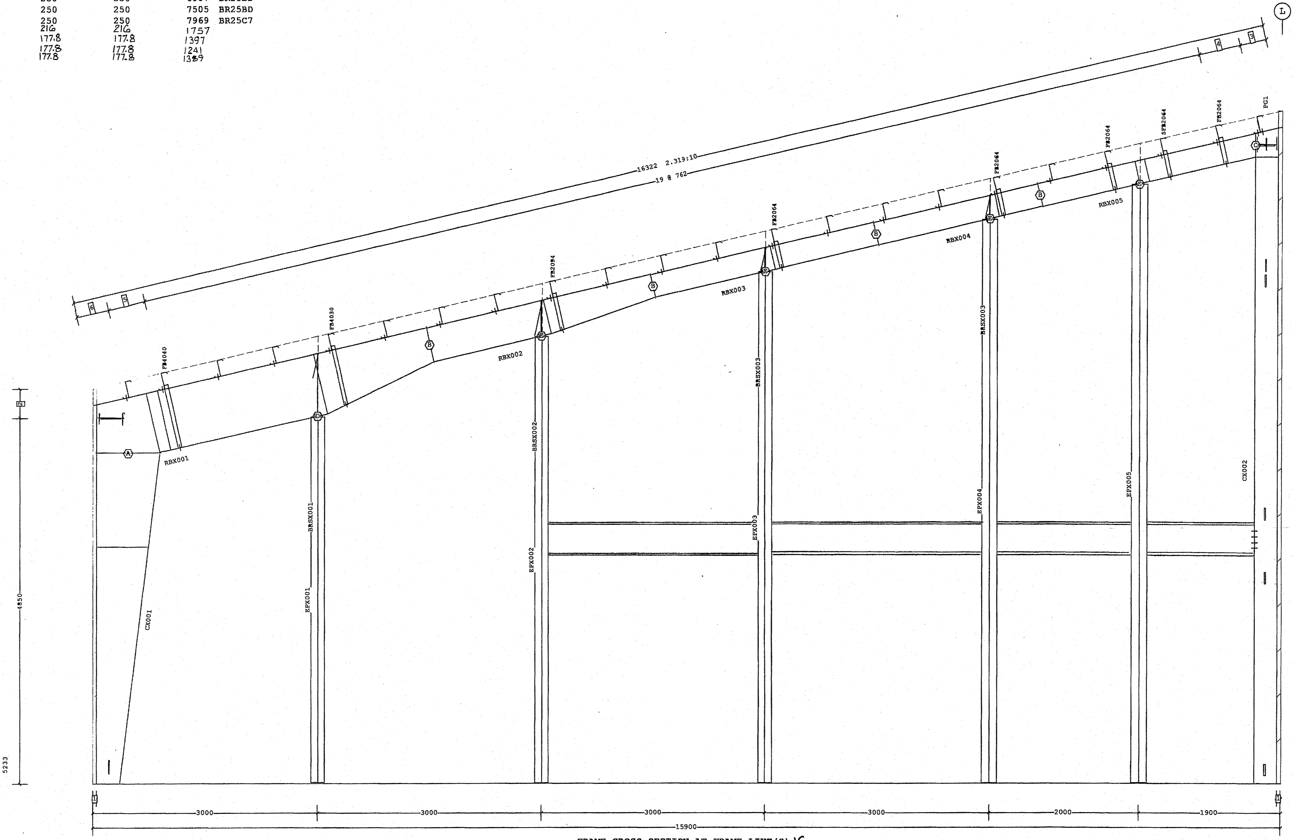
FRAME CROSS SECTION AT FRAME LINE(S) 1G
