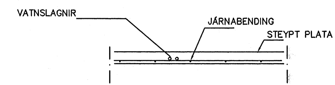
LAGNIR, SNID, 1:20
