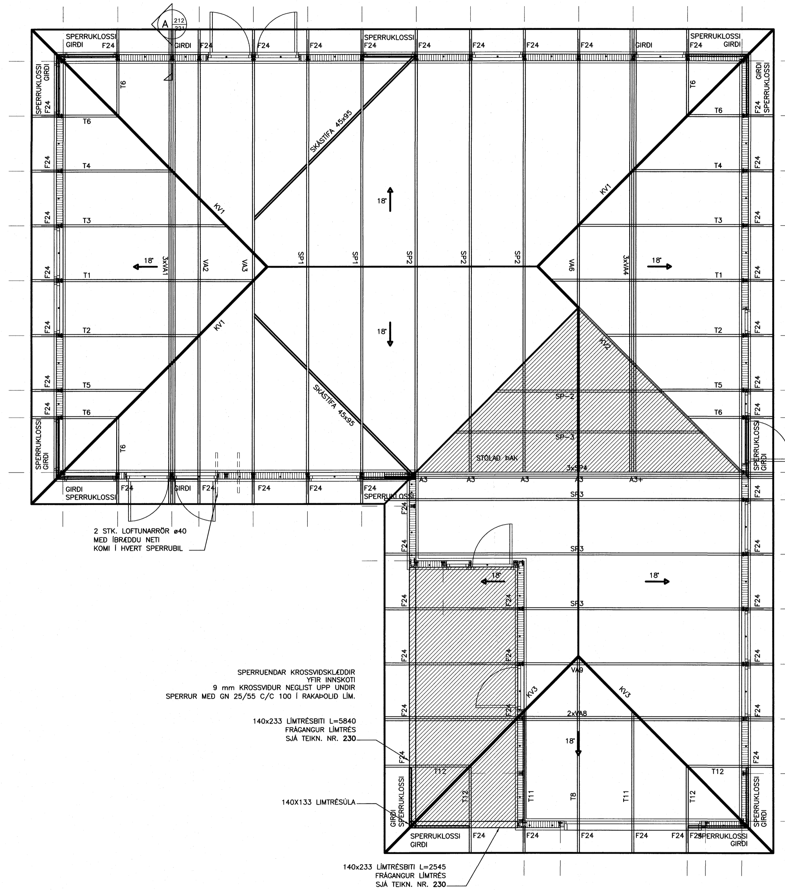
ÞAKPLAN MKV. 1:50
