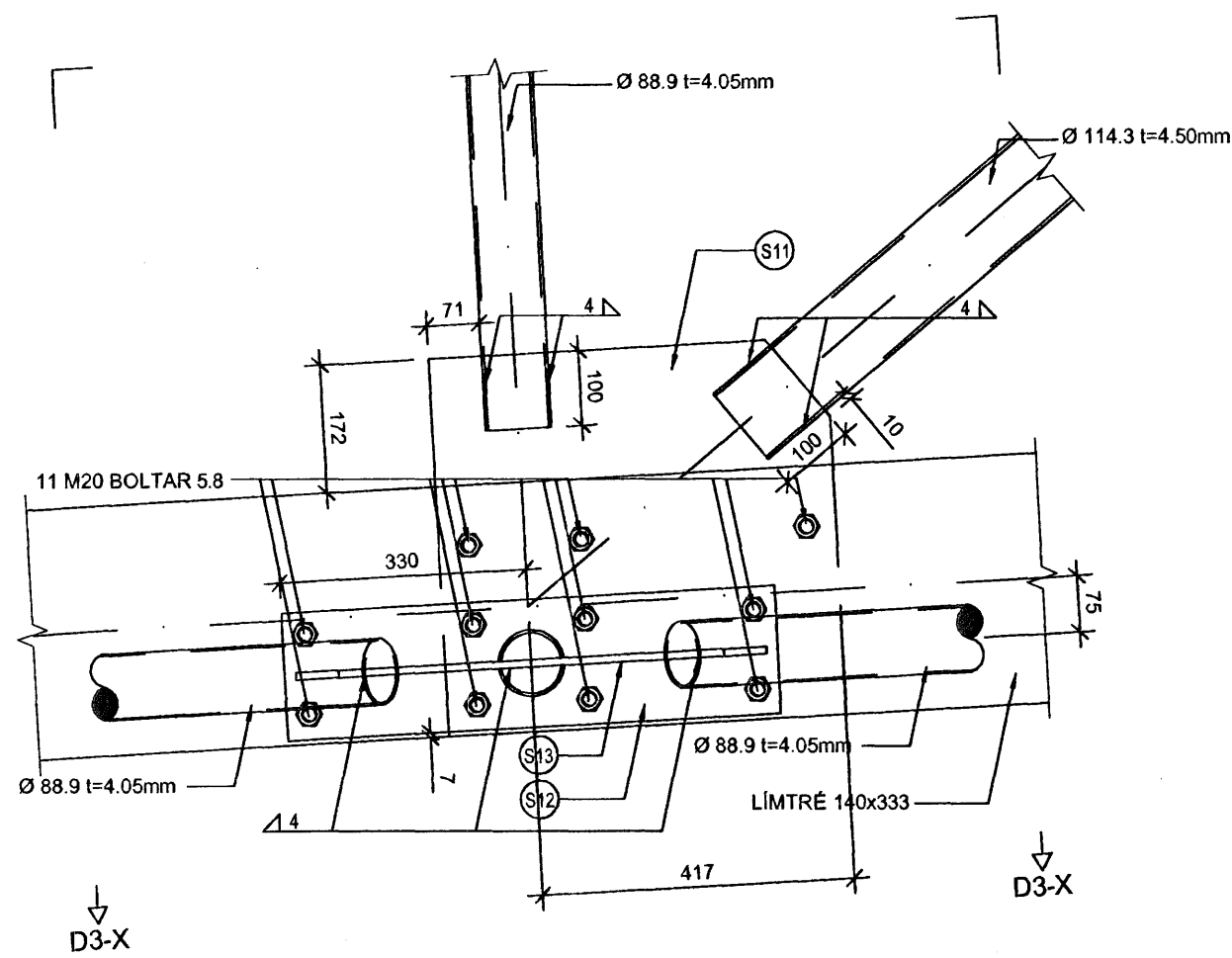
05 BH/2 SNID 1:10
