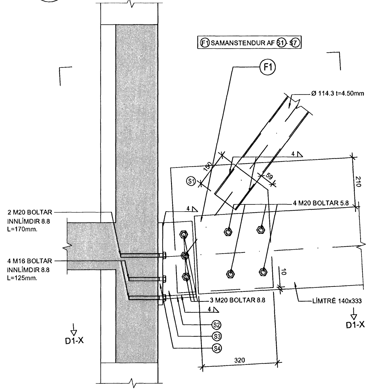
01 BH/2 SNID 1:10
