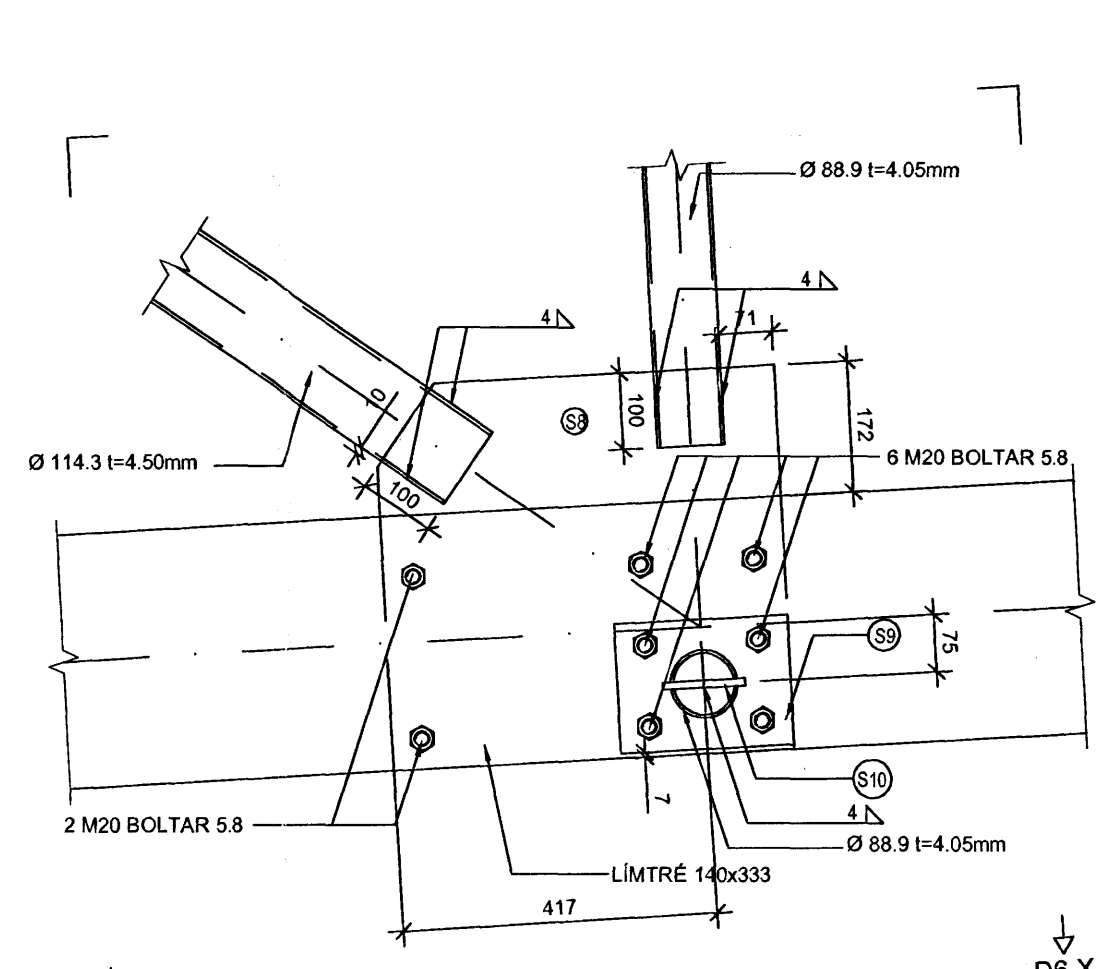
06 BH/2 SNID 1:10
