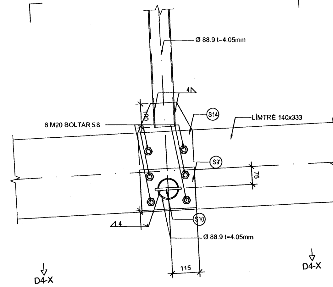
04 BH/2 SNID 1:10
