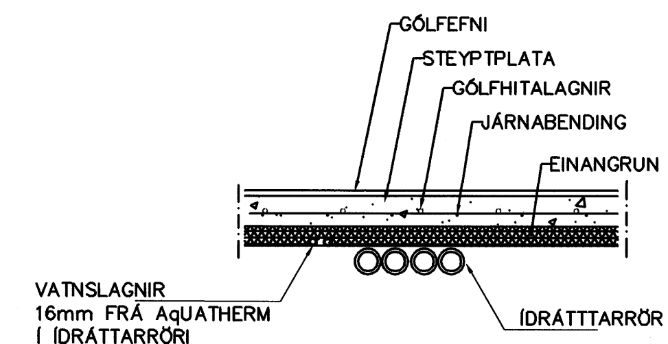
LAGNIR, SNID, 1:20
