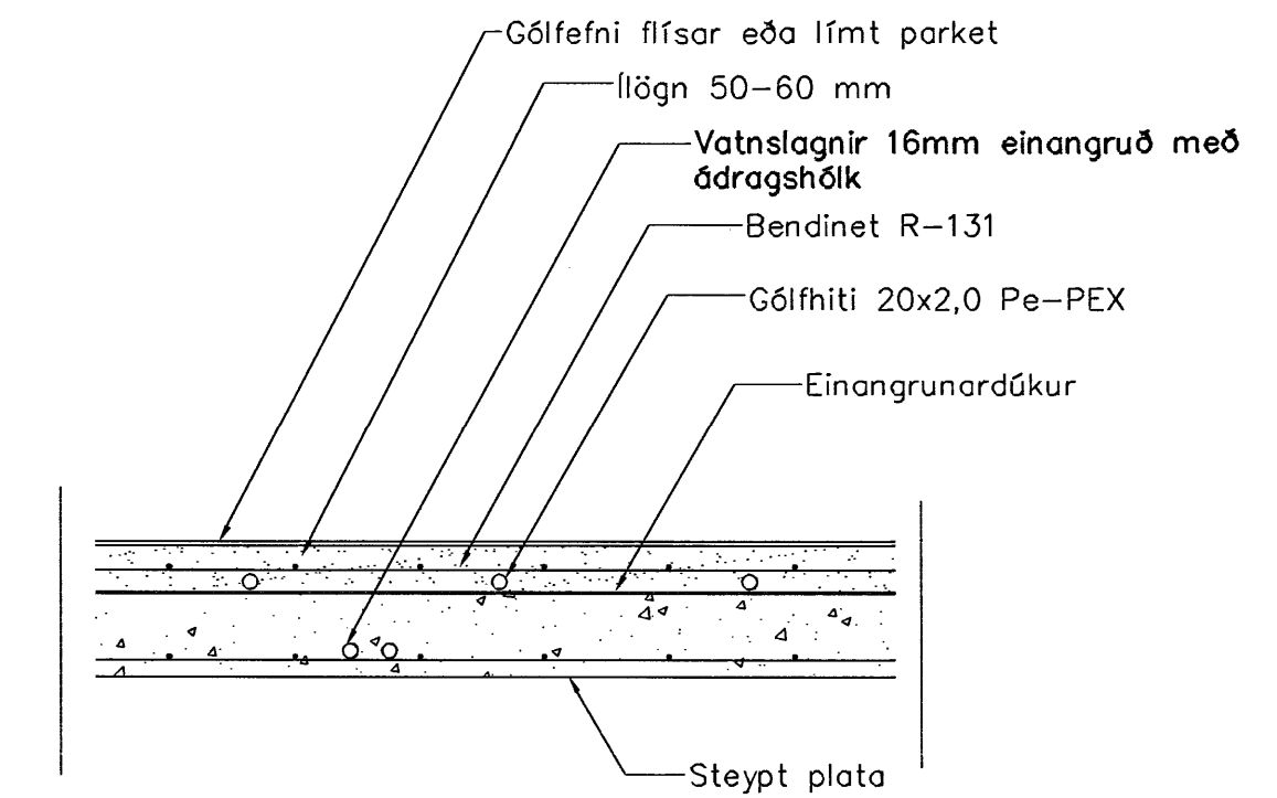
LAGNIR, SNID, 1:20
