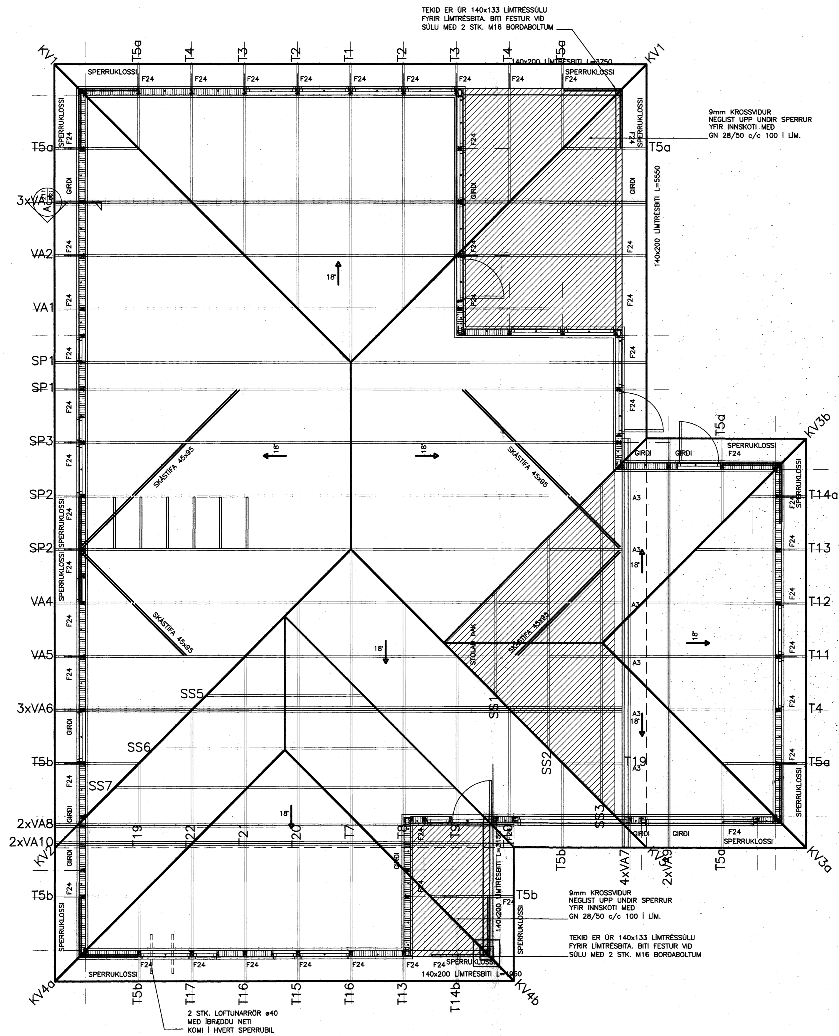
ÞAKPLAN MKY. 1:50
