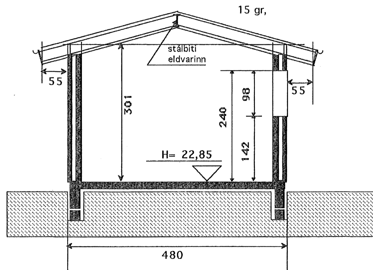
SNID B-B
