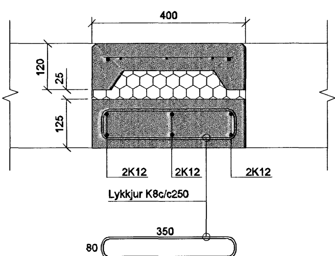
C-108 SNID. 1:10
