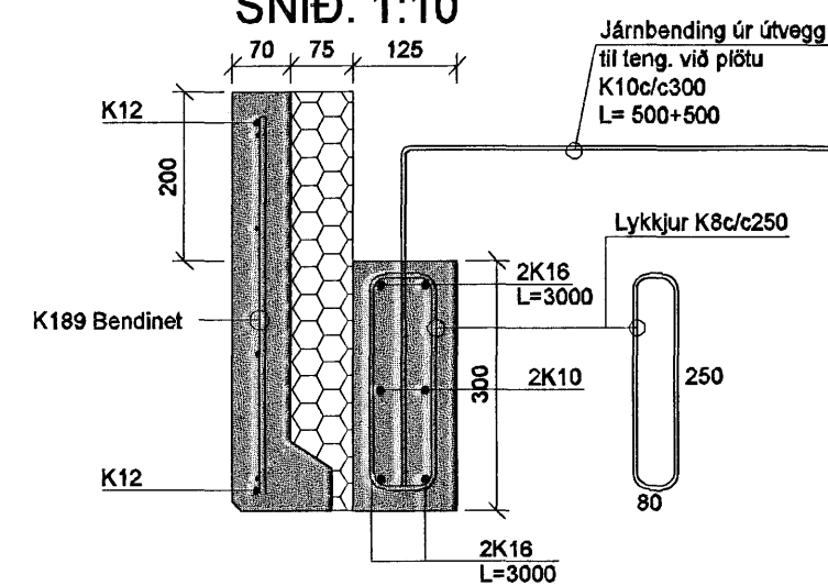
H-108 SNID. 1:10
