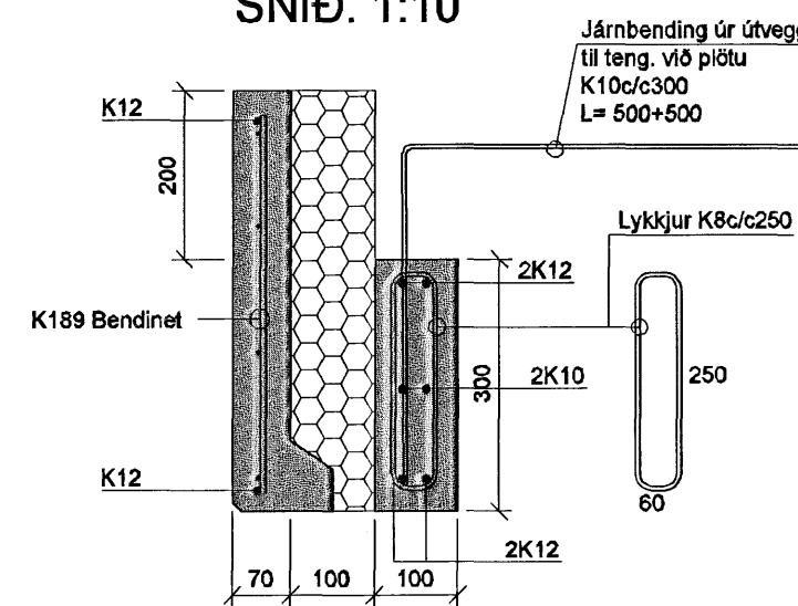
F-108 SNID. 1:10
