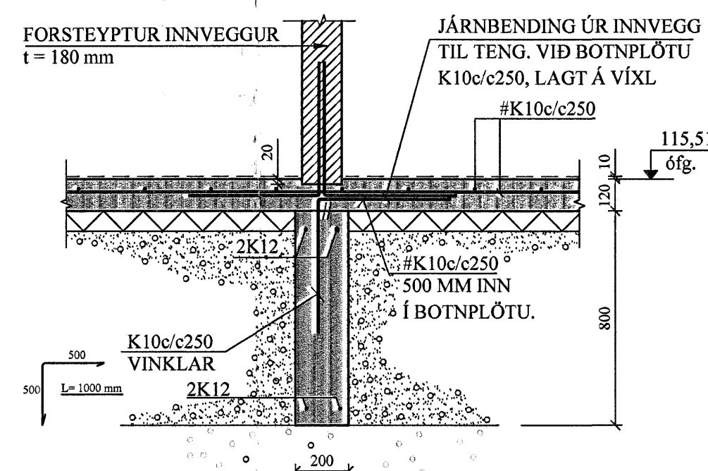
C2 SNIB. 1:20
