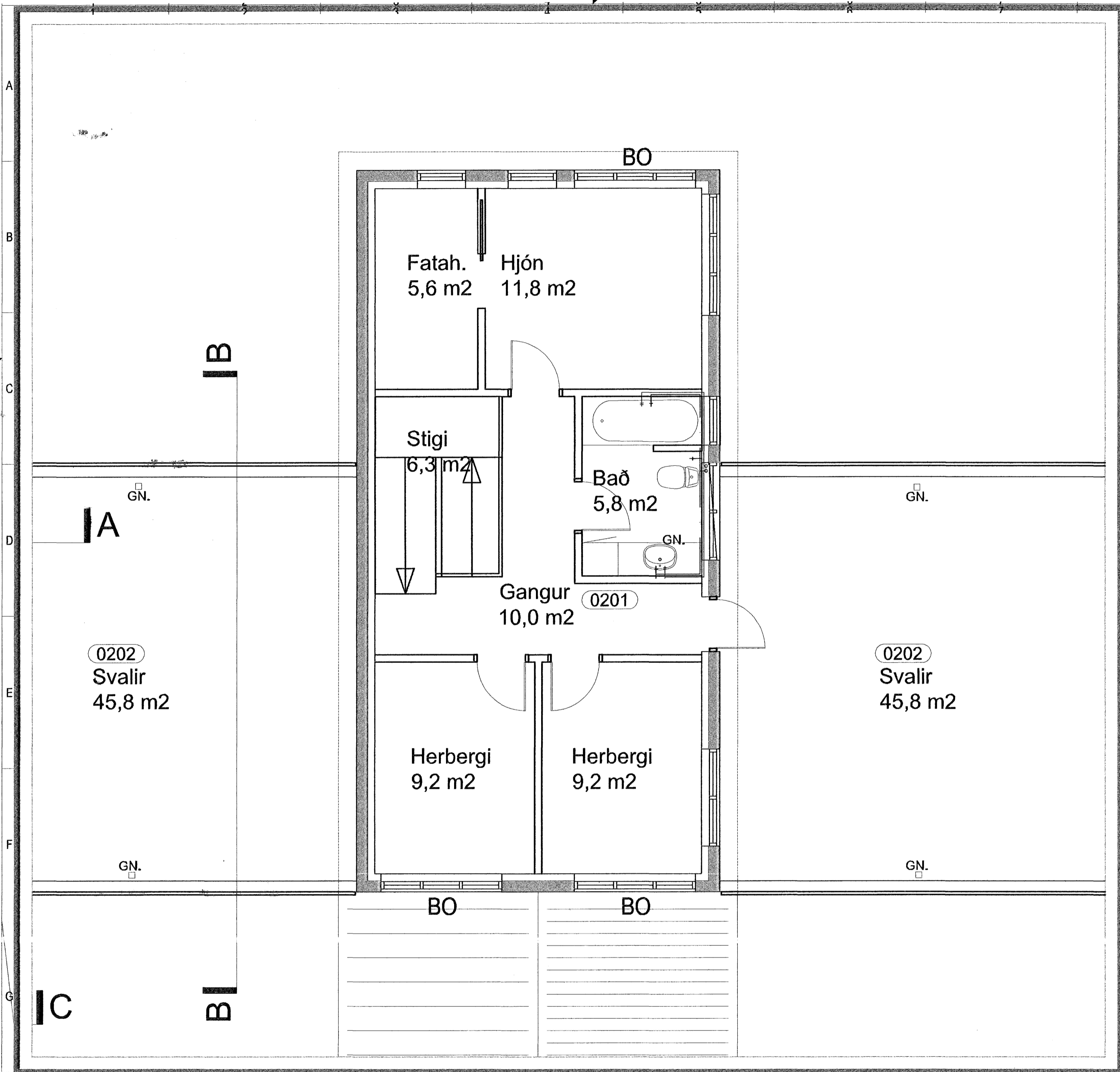
Plan 1:50.
