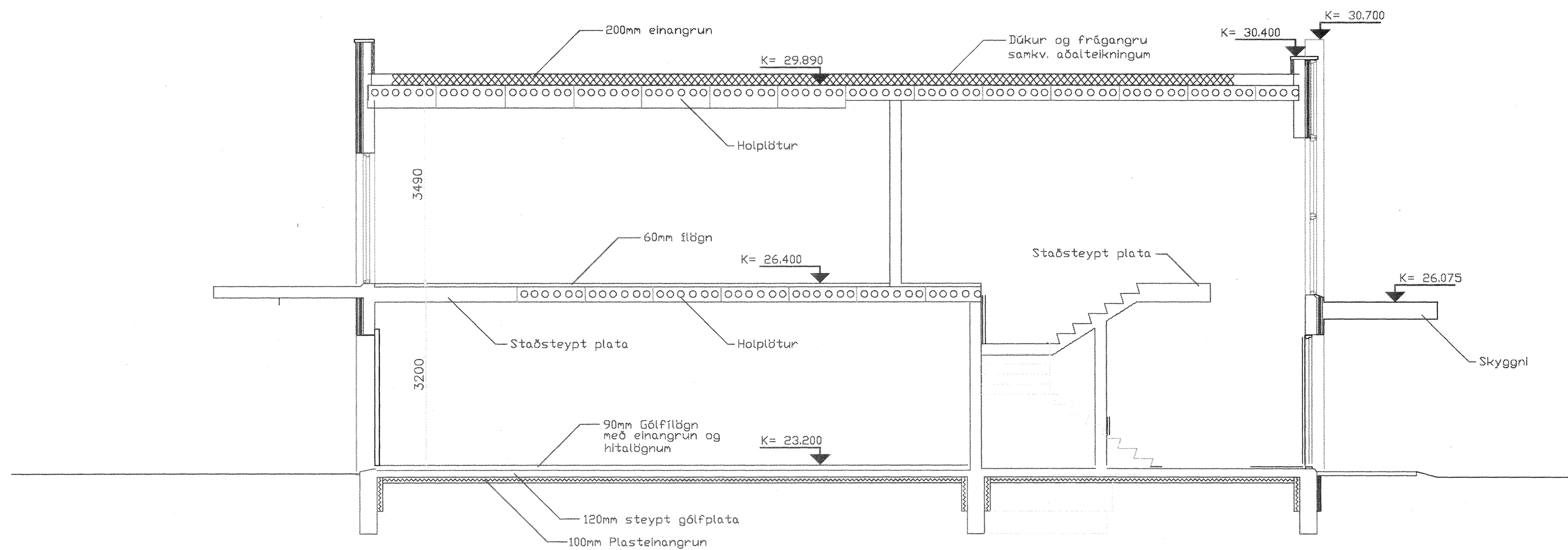
SNID H - H Mkv. 1: 50
