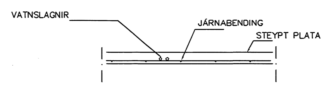
LAGNIR, SNID, 1:20
