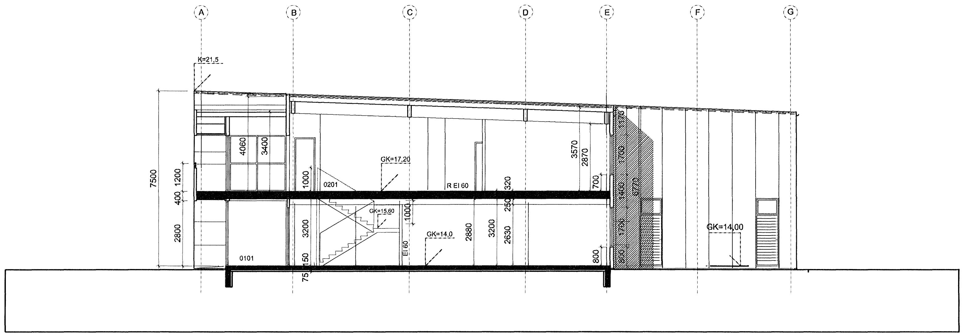
SNEIÐING C-C, M: 1/100.
