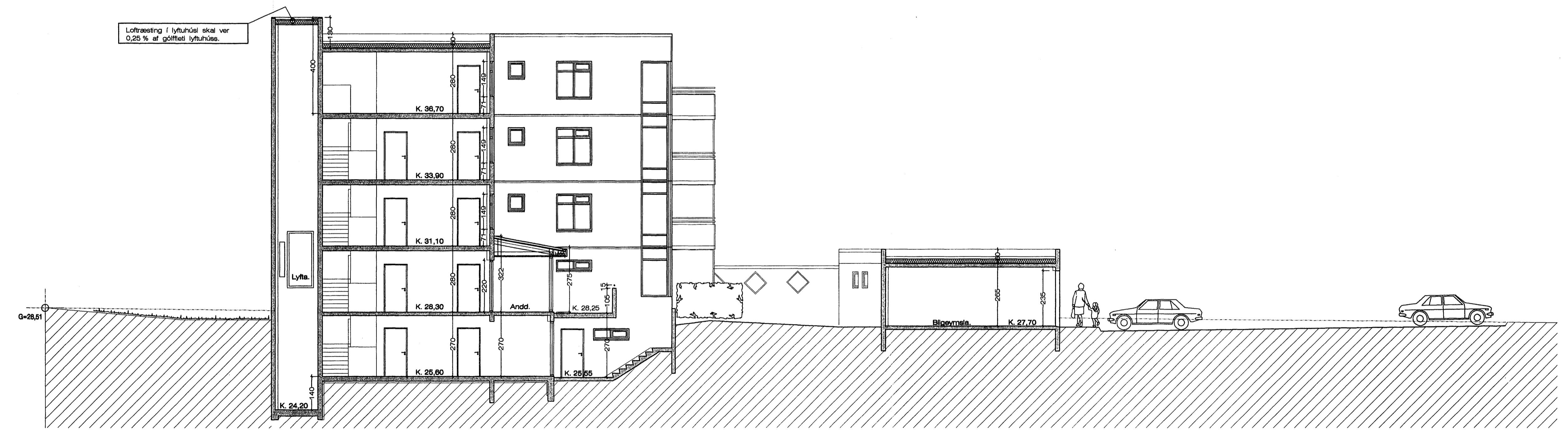
Sneiðing. B - B 1 : 100
