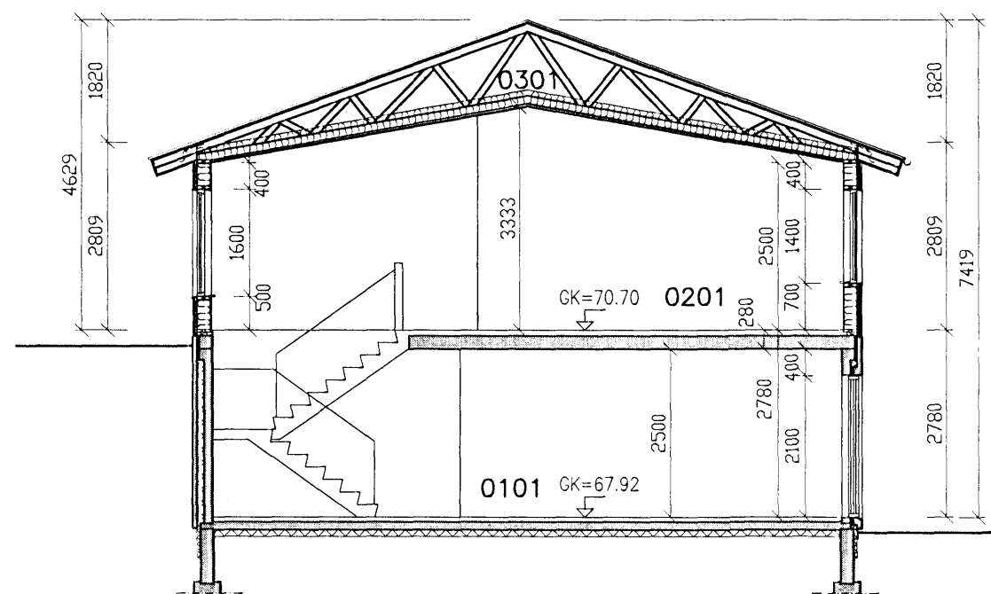
SNID 4-4 1:100
