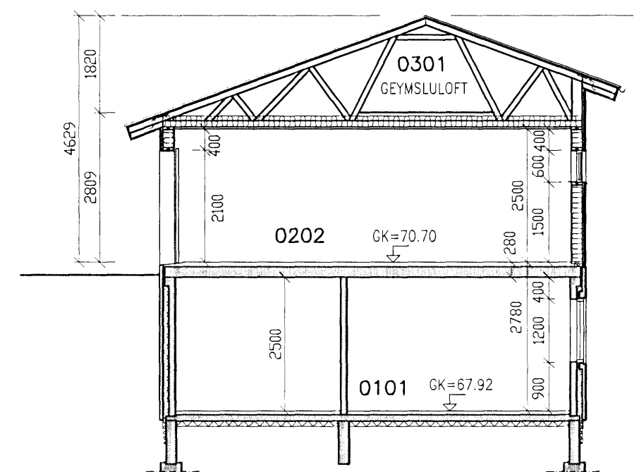
SNID 6-6 1:100
