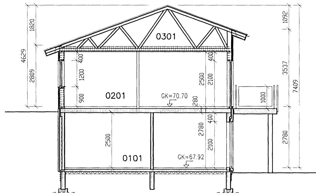
SNID 2-2 1:100
