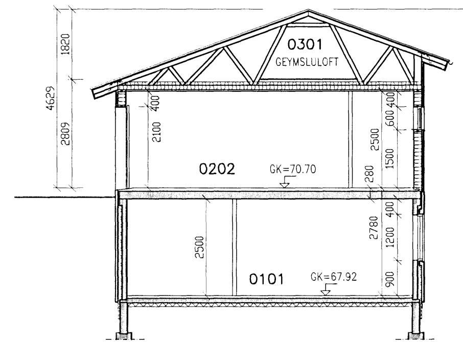
SNID 3-3 1:100
