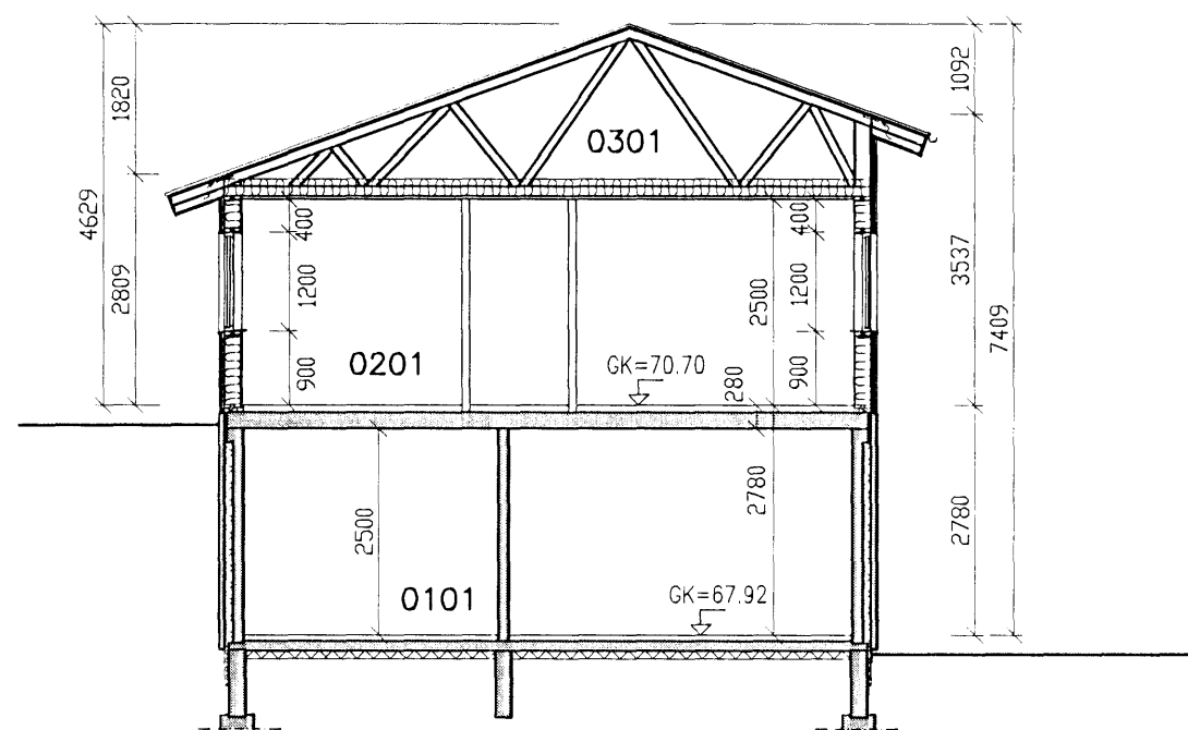
SNID 5-5 1:100
