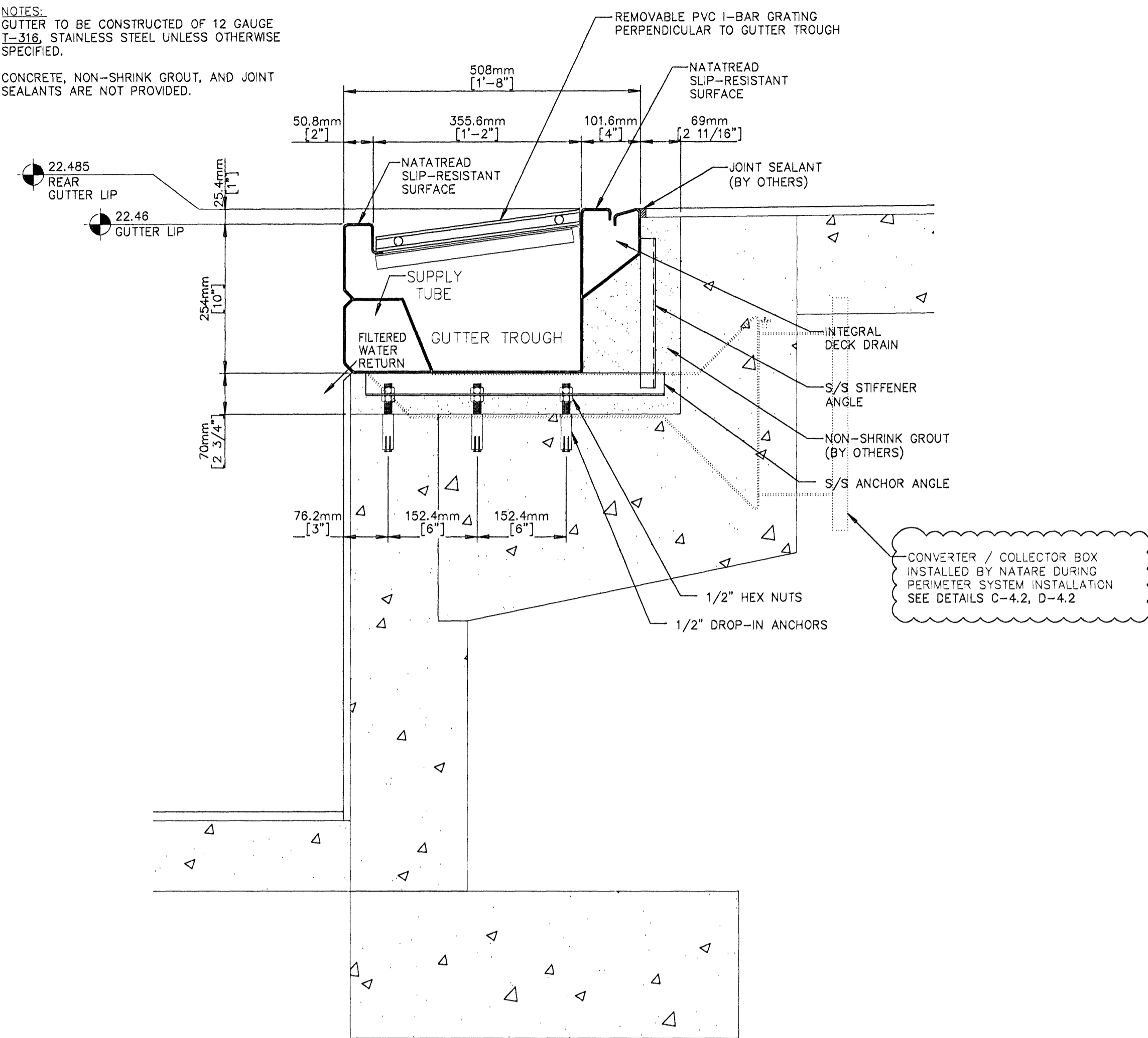
A 4.2 TRAINING POOL SECTION
