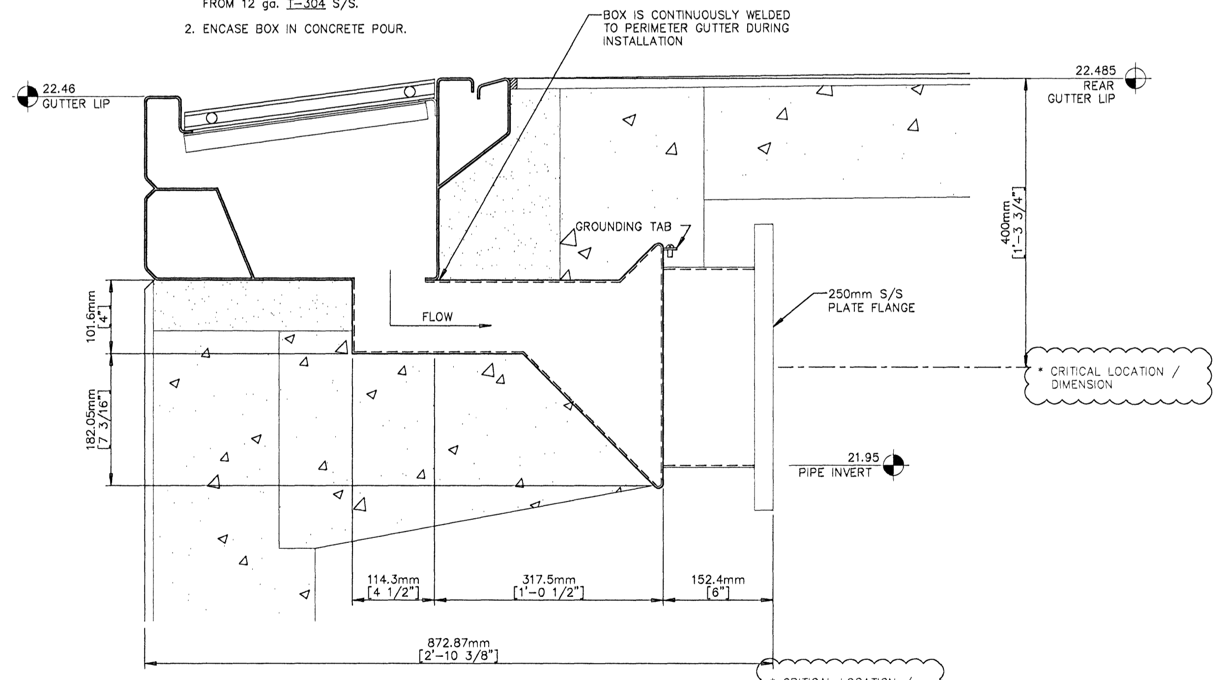
D 4.2 250mm GUTTER COLLECTOR BOX QTY.: 2 REQ'D.
