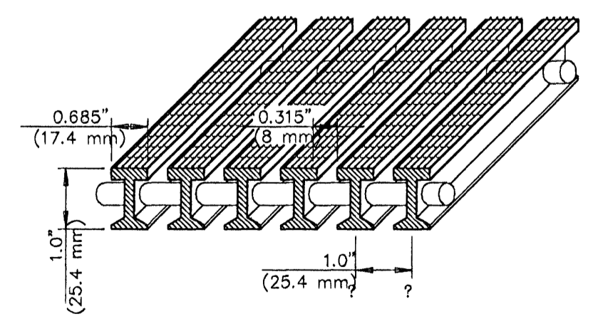
B 4.2 PVC I-BAR GRATING COLOR: WHITE
