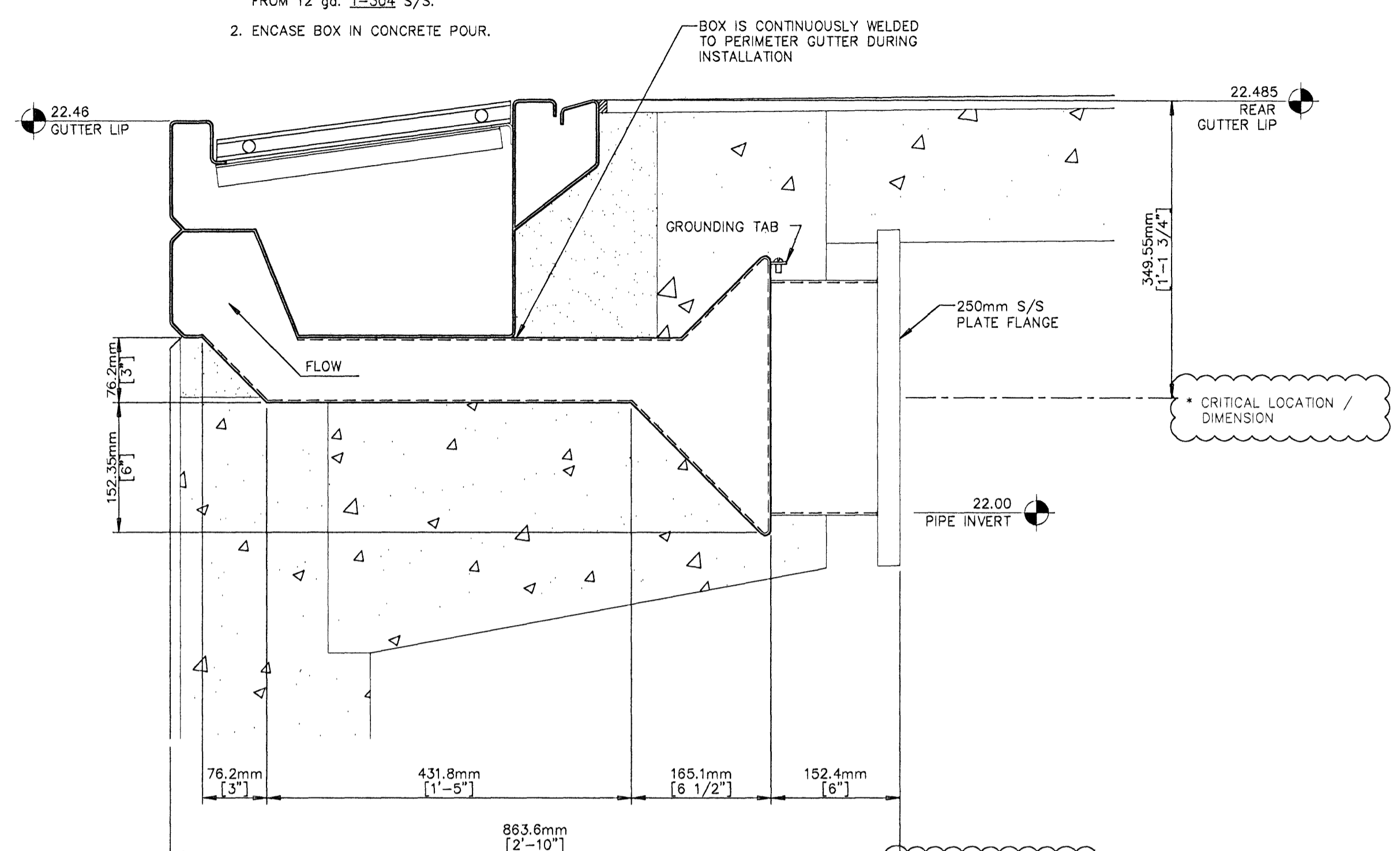
C 4.2 250mm SUPPLY CONVERTER BOX QTY.: 1 REQ'D.
