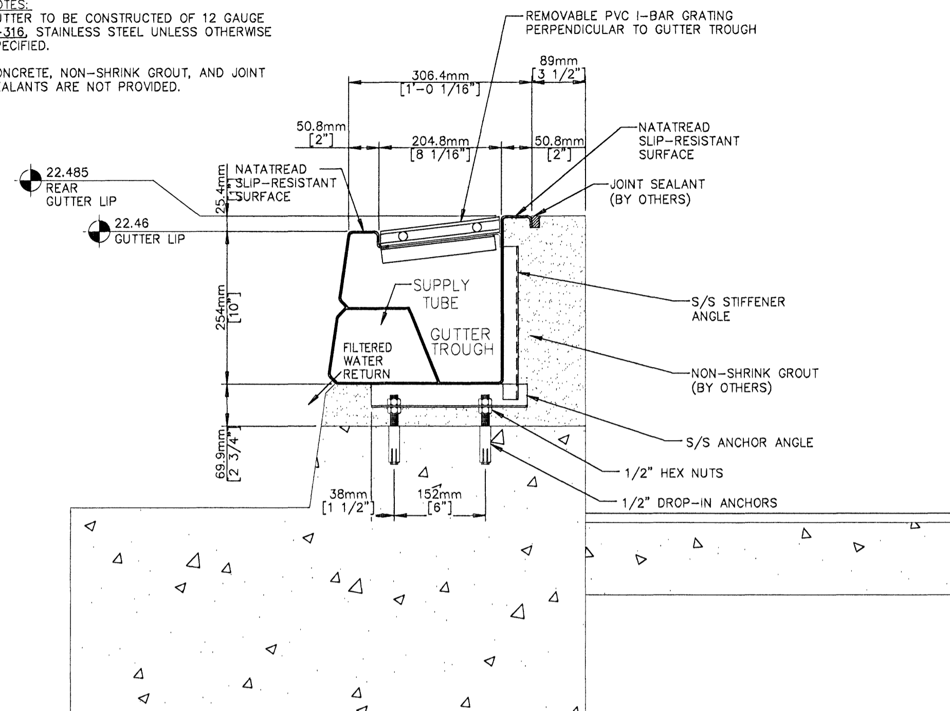
TYPICAL HOT POT SECTION
