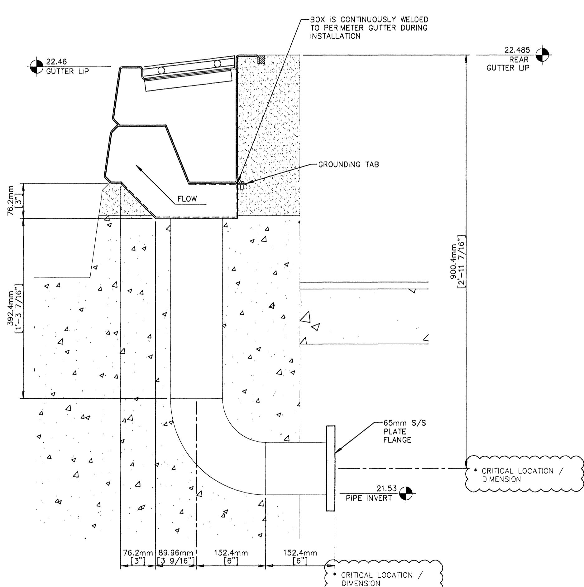
(C) 6.2 65mm SUPPLY CONVERTER BOX
