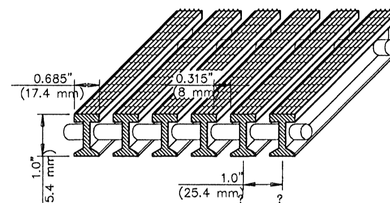
(B) 6.2 PVC I-BAR GRATING COLOR: WHITE
