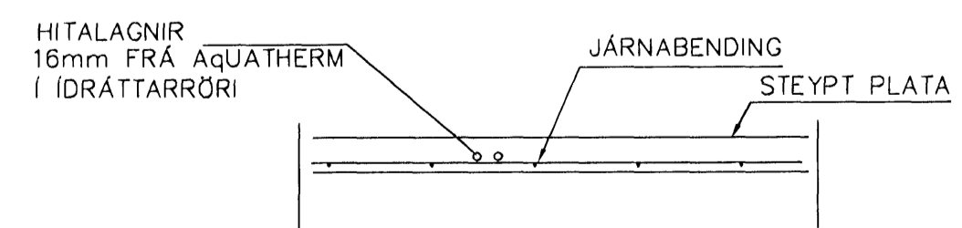
LAGNIR, SNID, 1:20
