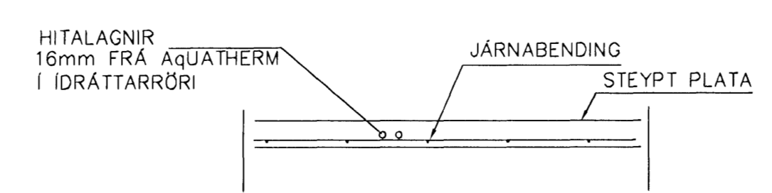
LAGNIR, SNID, 1:20
