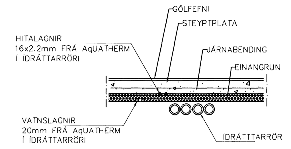
○ LAGNIR, SNID, 1:20
