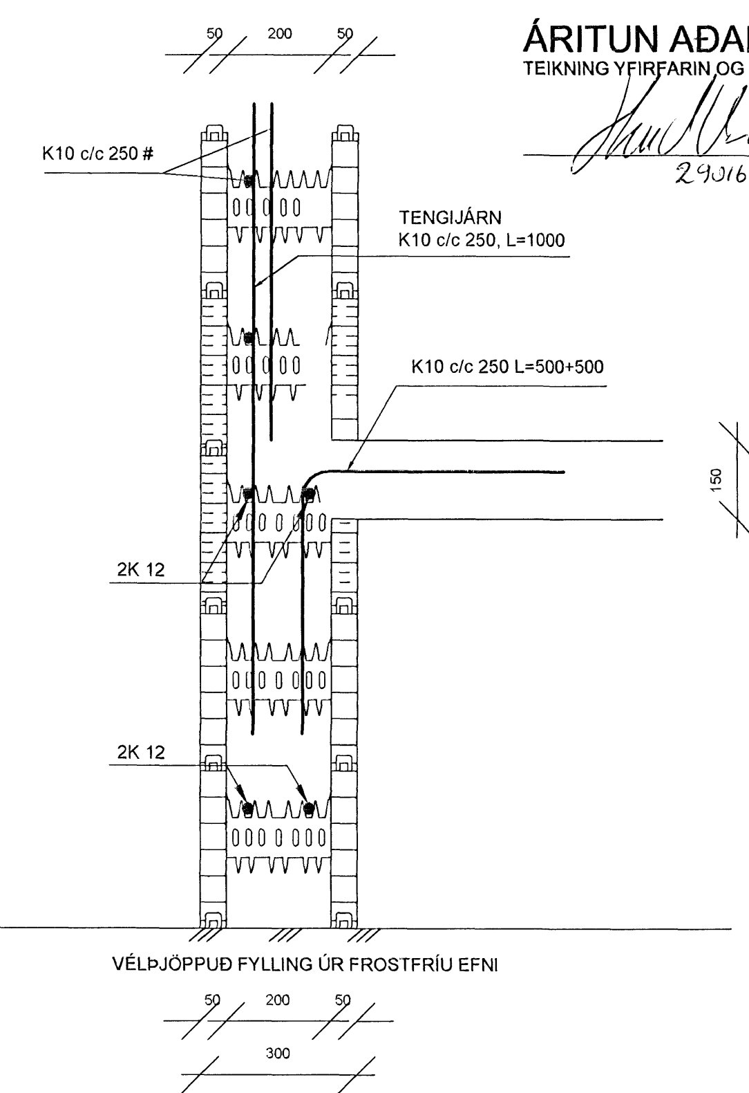
SNID C 1:10
