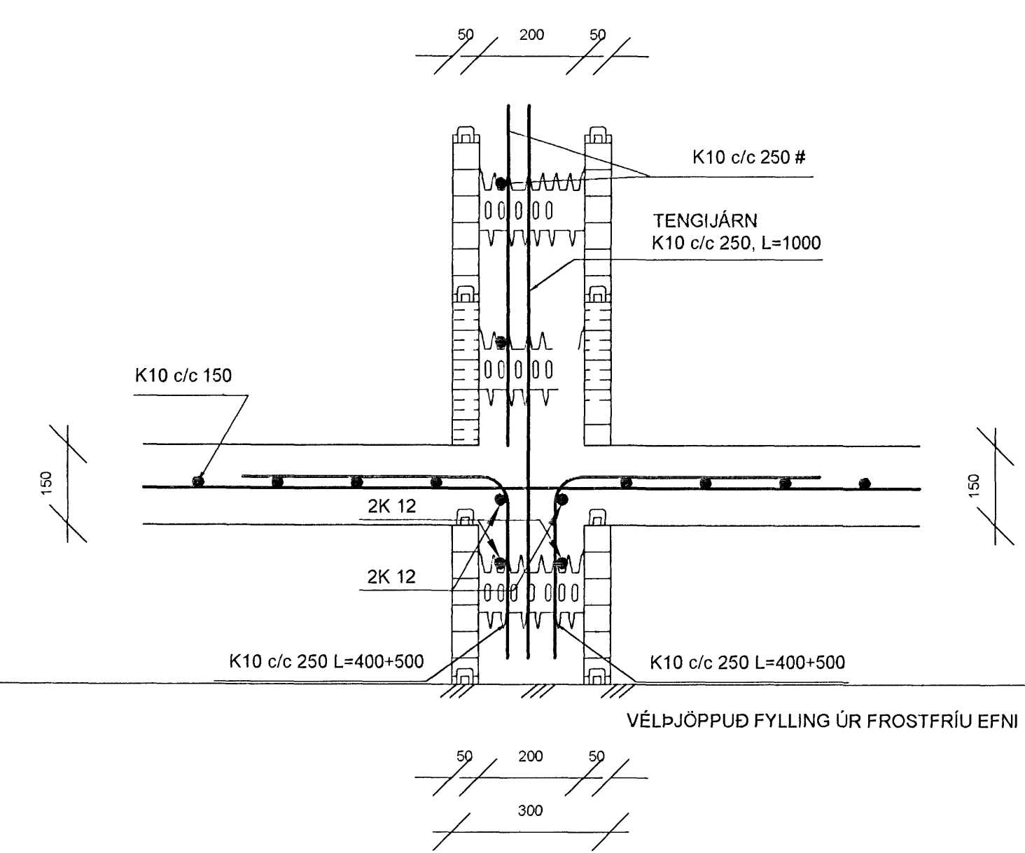
SNID C 1:10
