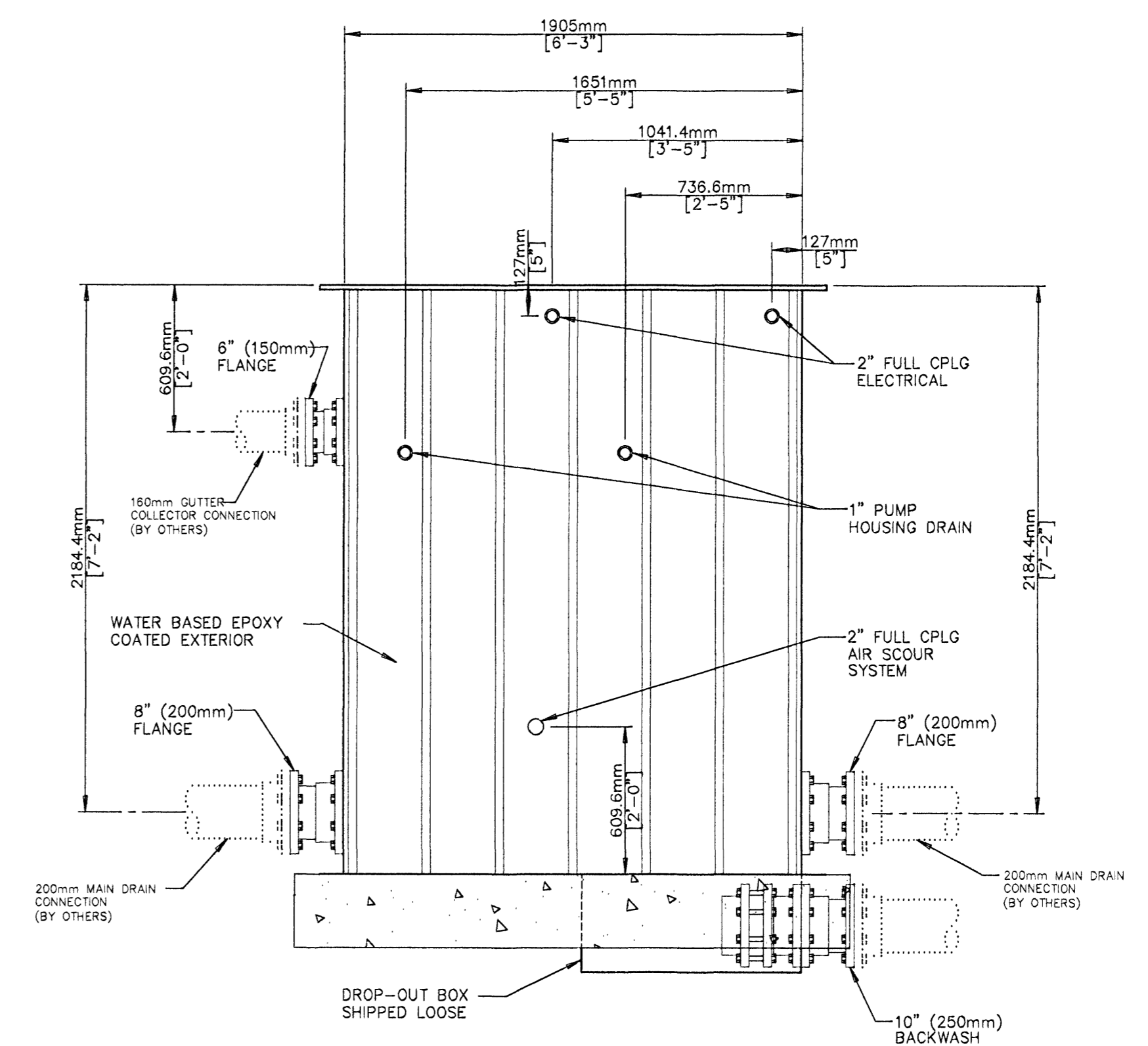
D 8.2b FILTER ELEVATION
