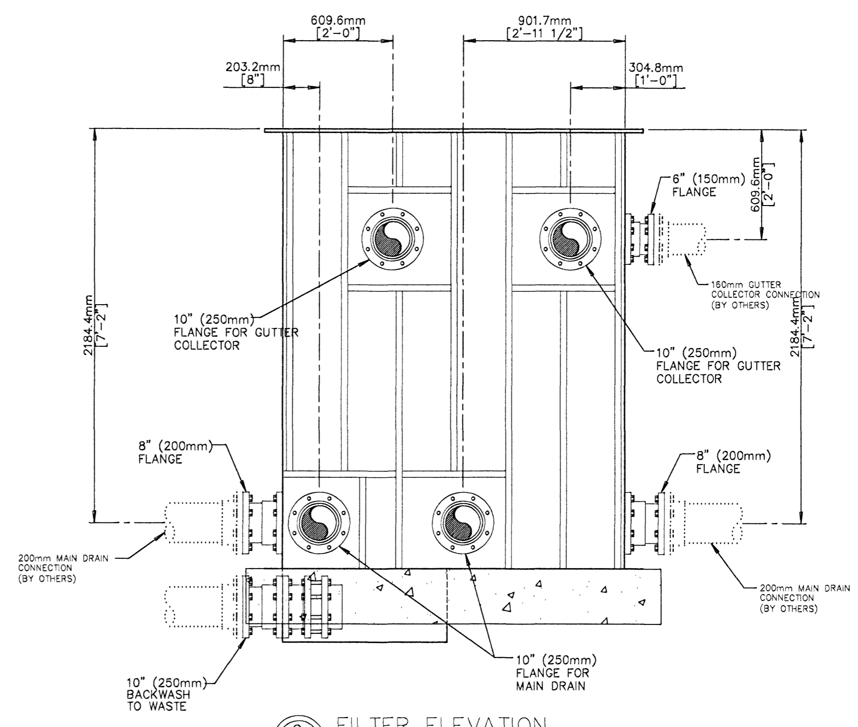
C 8.2b FILTER ELEVATION
