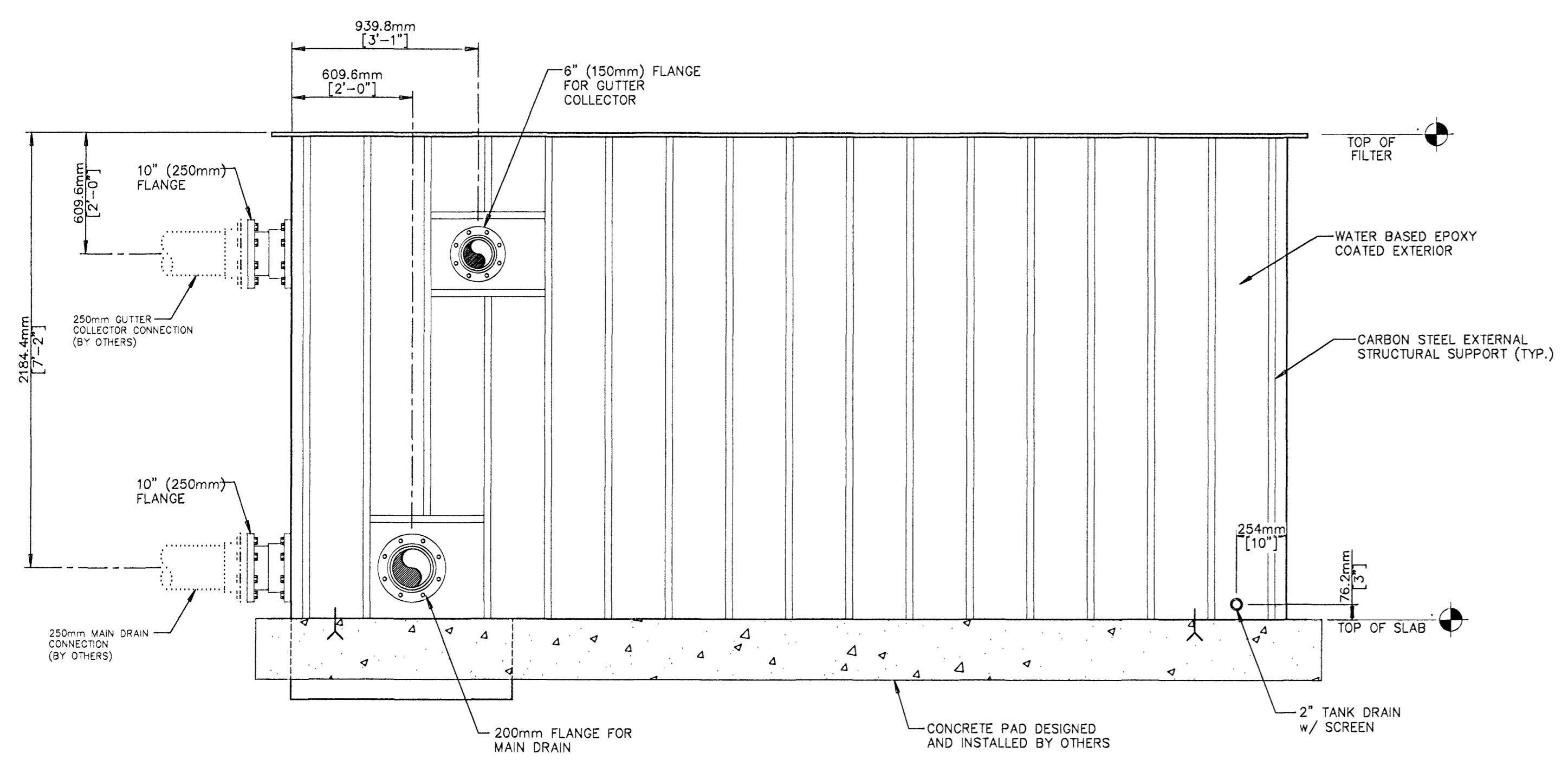
B 8.2b FILTER ELEVATION
