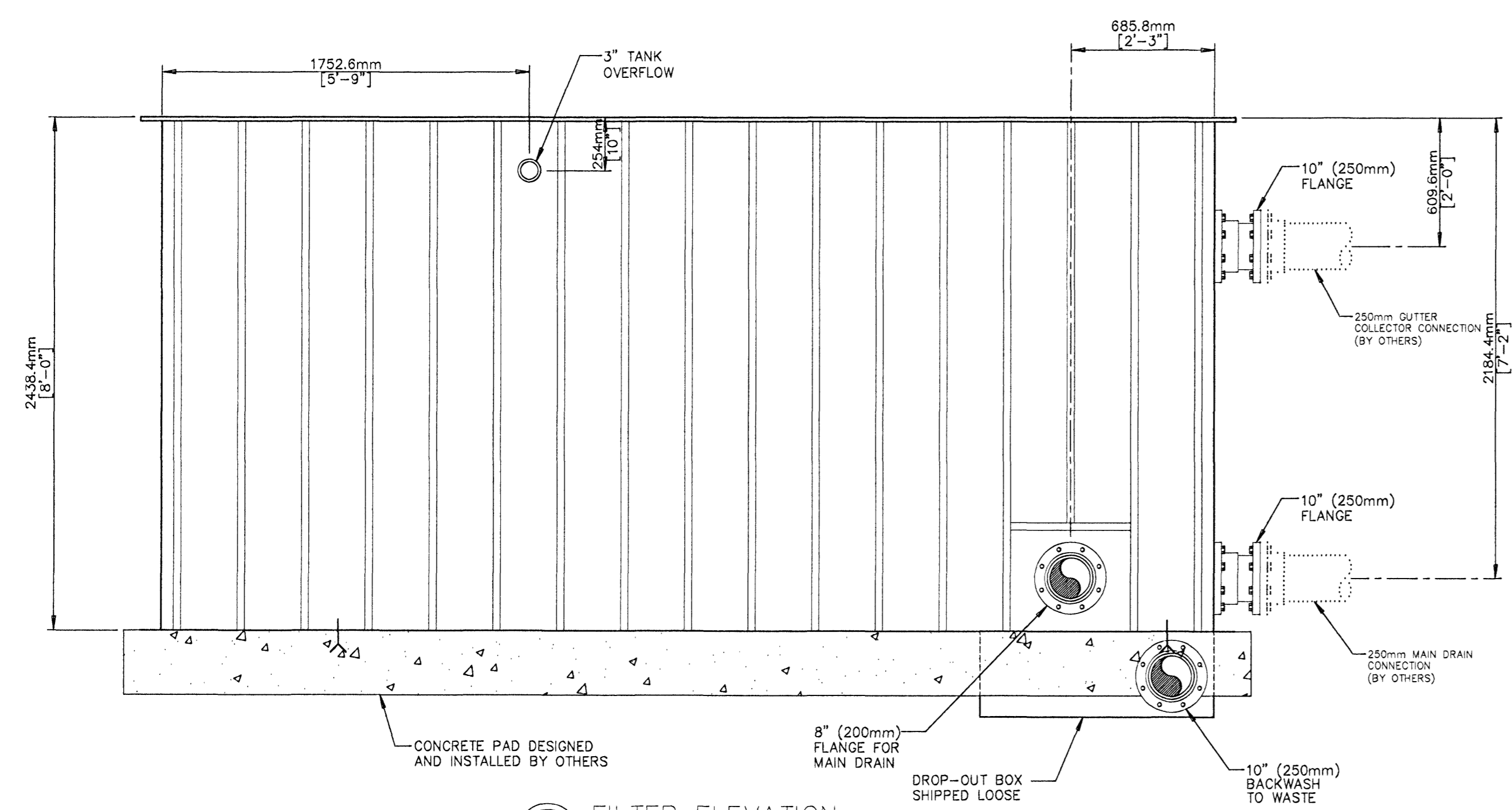
A 8.2b FILTER ELEVATION
